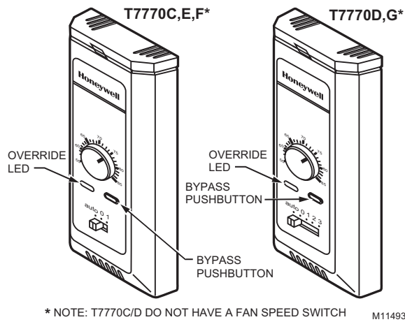
Fig. 2. LED and bypass pushbutton locations.
