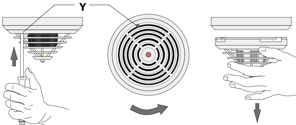
Figure 5.2: Detector removal (locked detector head)
