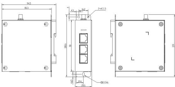
Figure 2-1 Outline dimensions for ICA417
