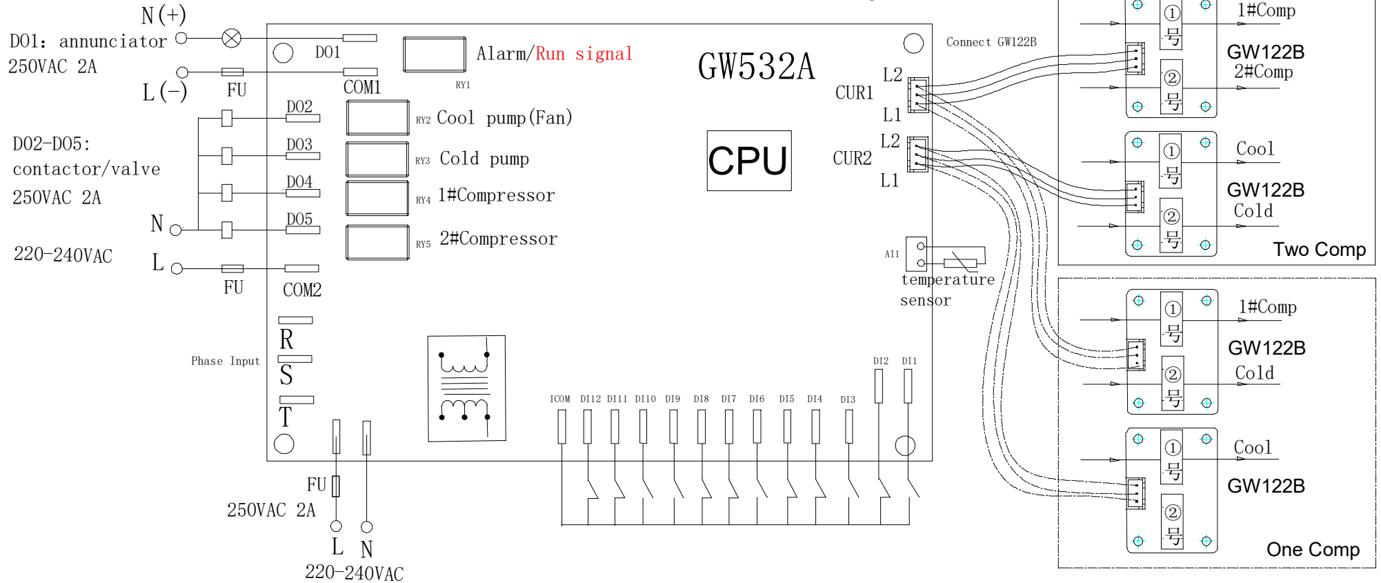
X1. GW532A. TY. F01M. Electrical Connection Diagram
