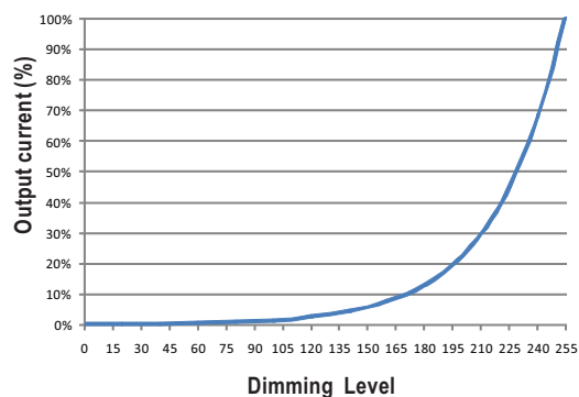
Dimming characteristics
