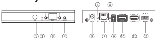
Figure 1: Transmitter (TX)
