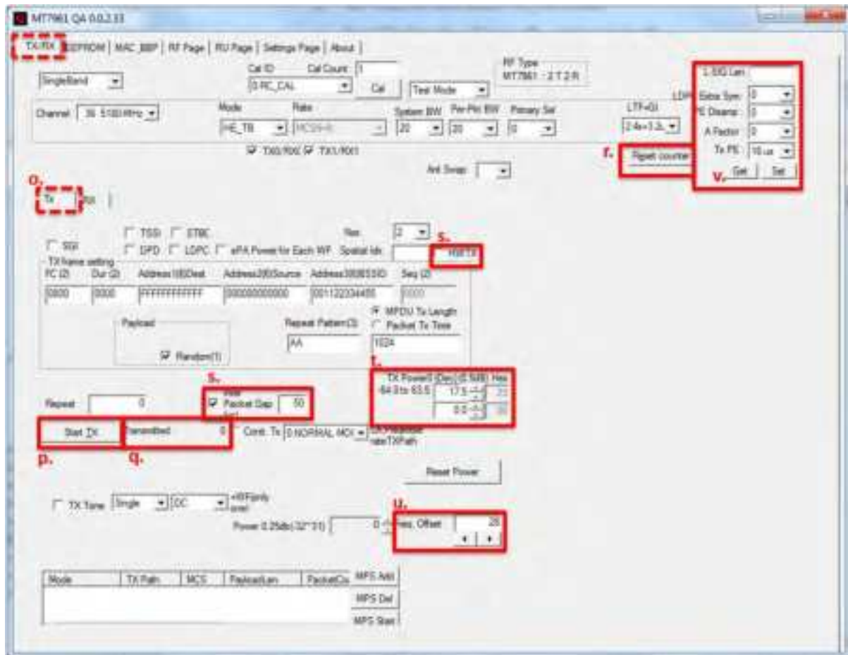
An example of 2TX transmitting HE_TB BW20 RU26 index8 MCS11 infinite packets at 5180MHz.
