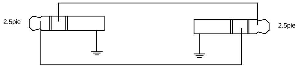
Figure 2-16 Cloning Cable Schematic
