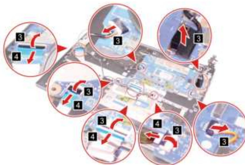
Figure 37. Disconnect cables
