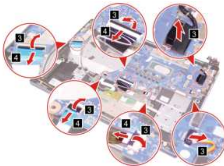
Figure 33. Disconnect cables
