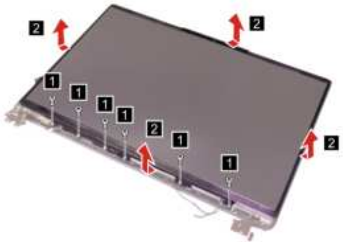
Figure 54. Remove the LCD bezel
