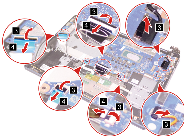
Figure 33. Disconnect cables
