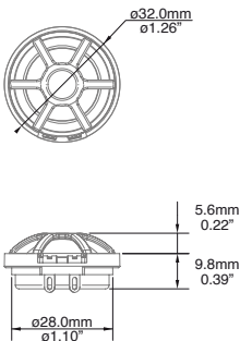
Without housing
