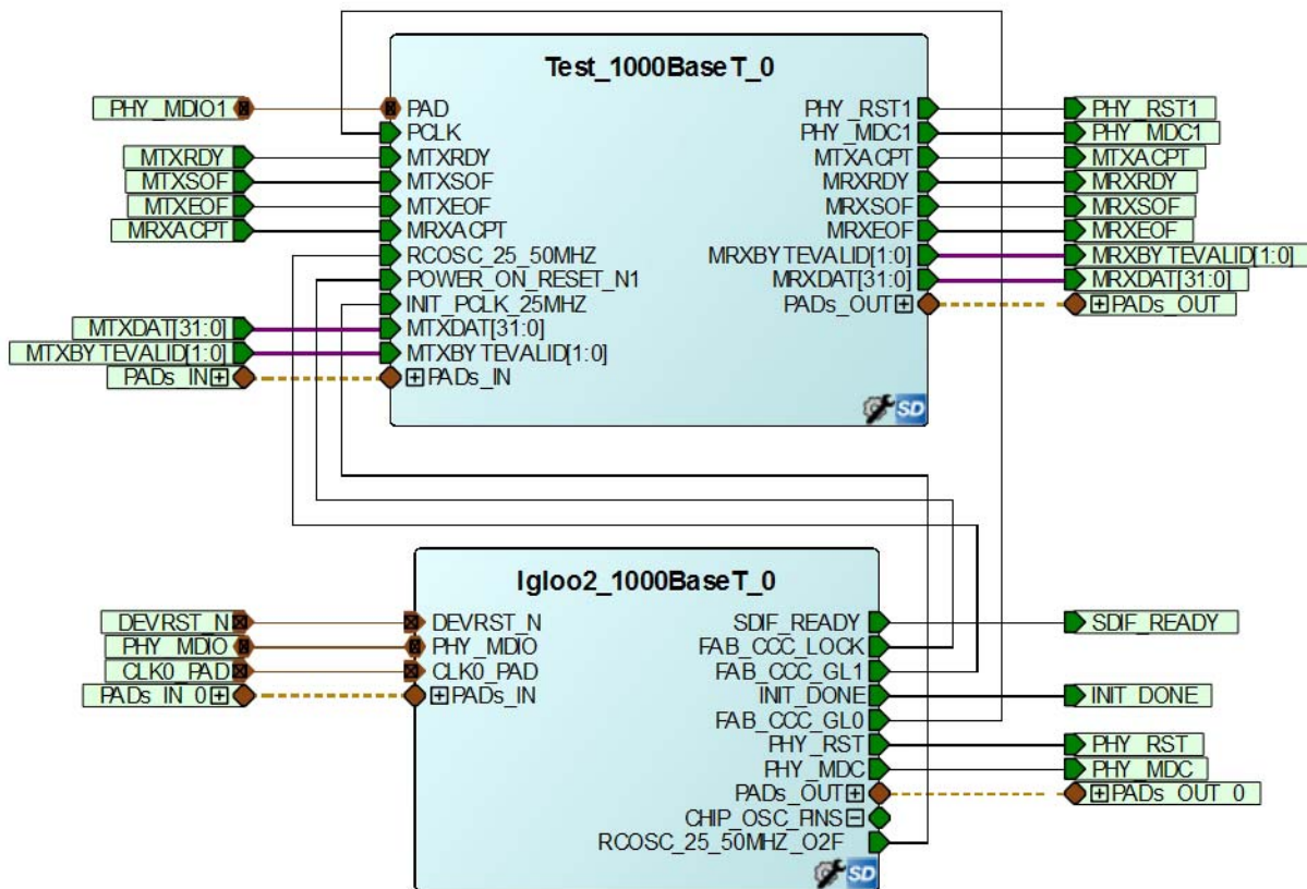
Figure 5 • Libero SmartDesign Top-Level Module
