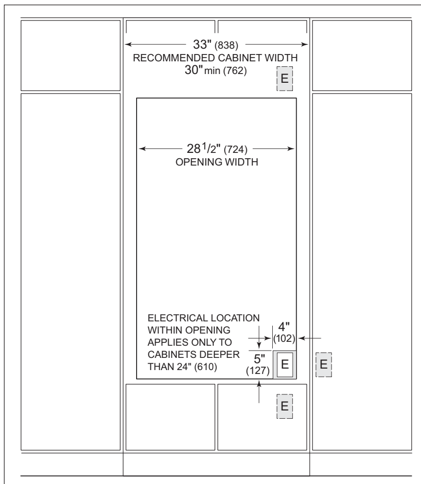
Figure 2-6. Front Cutout Dimensions and Electrical Placement
