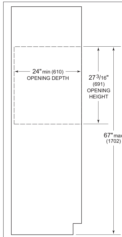
Figure 2-5. Side View
