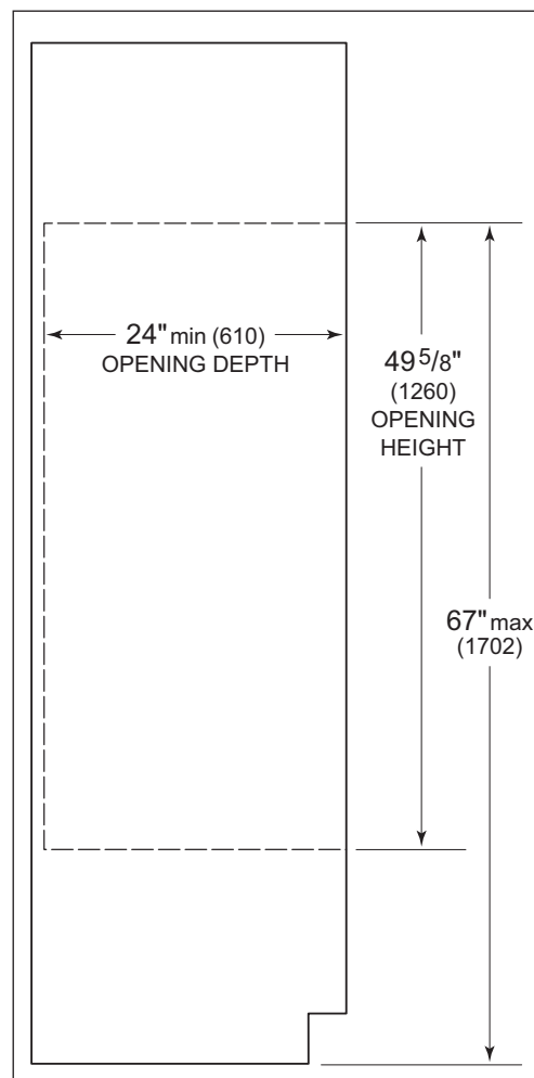
Figure 2-7. Side View
