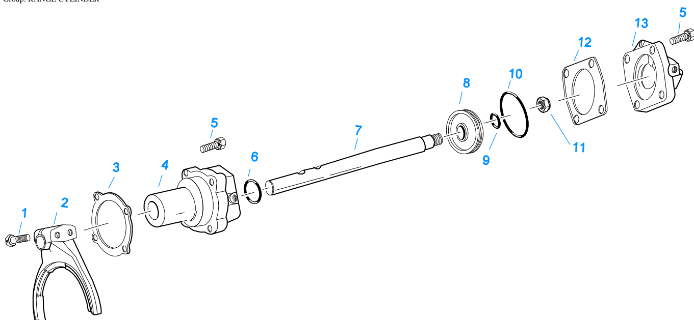
10462-4/92 Rng Cyl
