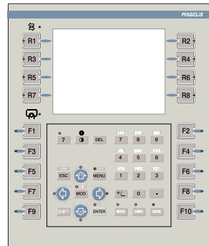
Figure 1-2: XBT-F 10"
