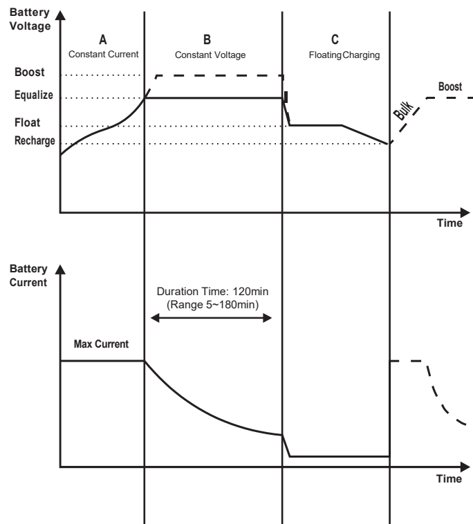
Battery Changing Stage Curve
