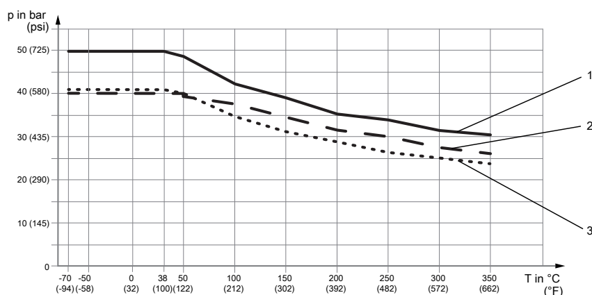
Fig. 14: Allowed process pressure as a function of process connection temperature
