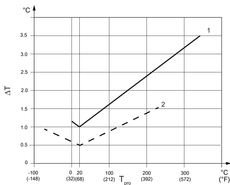
Fig. 11: Temperature accuracy
