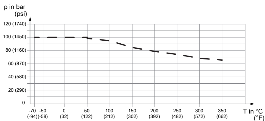
Fig. 16: Allowed process pressure as a function of process connection temperature, suitable for flange EN 1092-1 PN100
