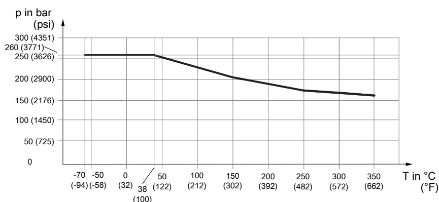
Fig. 18: Allowed process pressure as a function of temperature, suitable for process connection temperature, suitable for process connections with internal thread G and NPT
