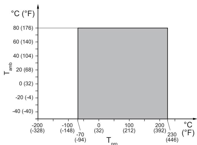
Fig. 21: Allowed medium and ambient temperatures
