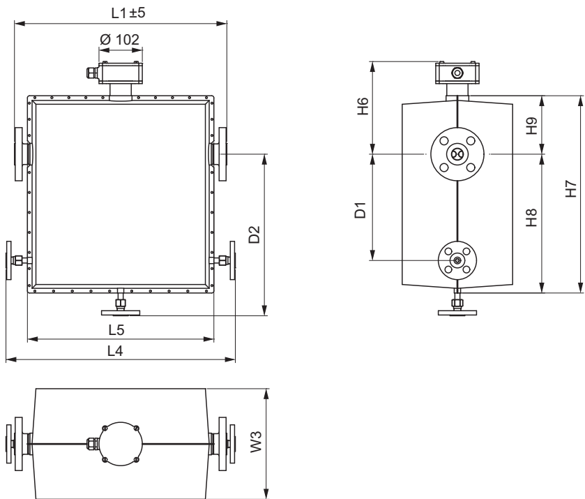
Fig. 24: Dimensions in mm
