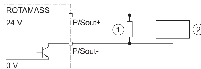
Fig. 31: Active pulse output connection P/Sout
