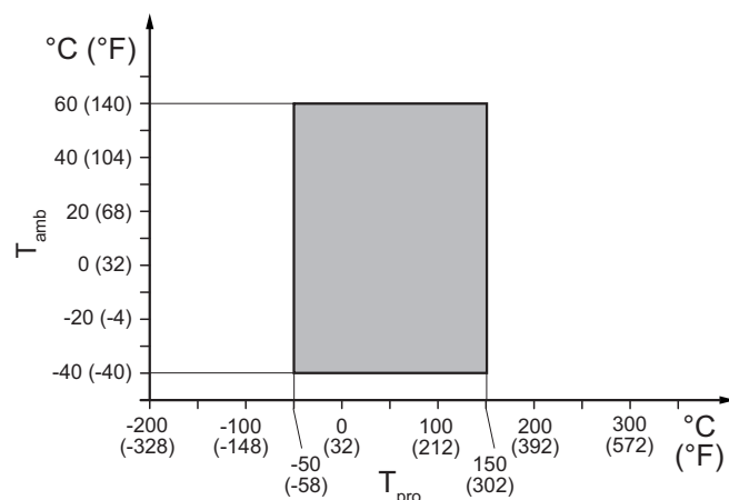
Fig. 19: Allowed medium and ambient temperatures, integral type
