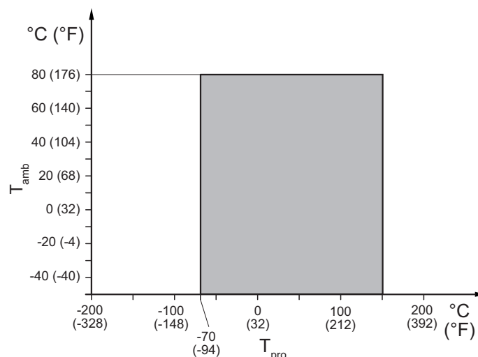
Fig. 20: Allowed medium and ambient temperatures, remote type
