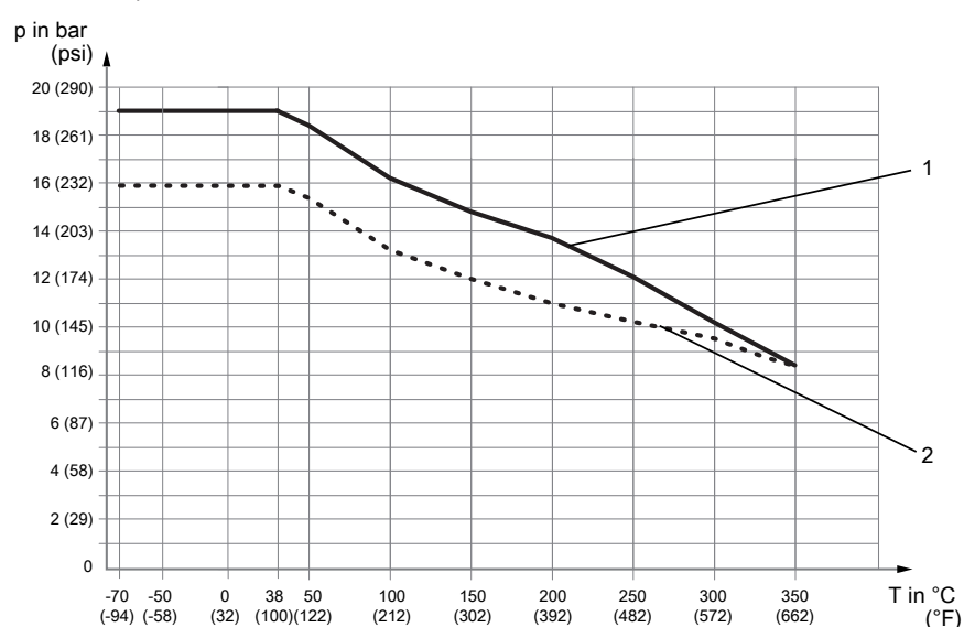
Fig. 13: Allowed process pressure as a function of process connection temperature
