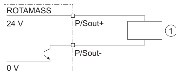
Fig. 36: Active status output connection P/Sout
