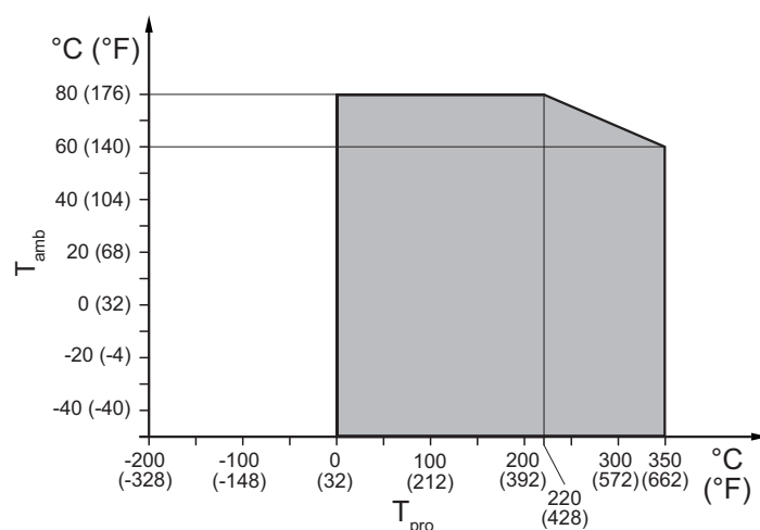
Fig. 22: Allowed medium and ambient temperatures
