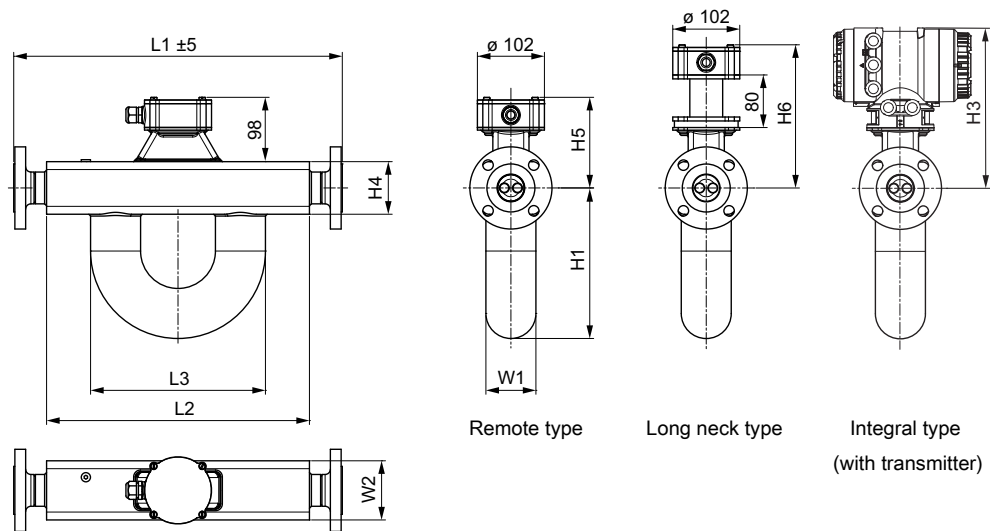
Fig. 24: Dimensions in mm
