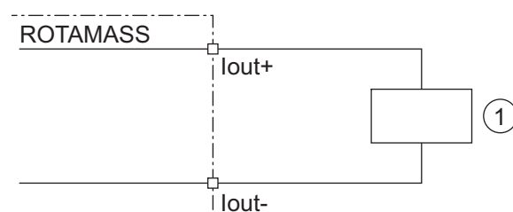
Fig. 28: Active current output connection Iout HART
