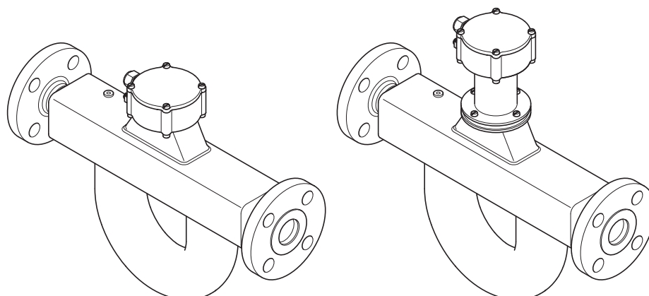
Fig. 23: Standard terminal box and long neck
