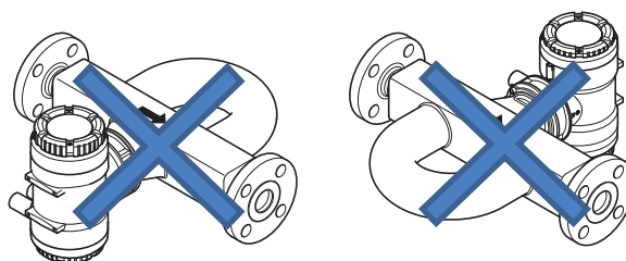
Fig. 12: Installation position to be avoided: Flow meter in sideways position
