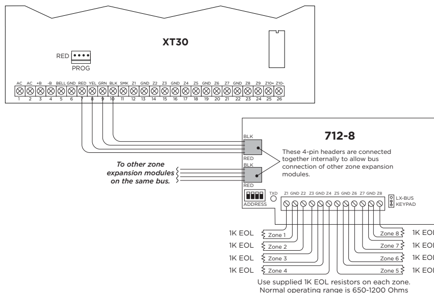
Figure 3: Wiring Diagram
