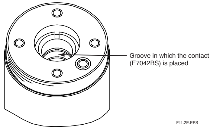
Figure 11.2 Installing the Contact
