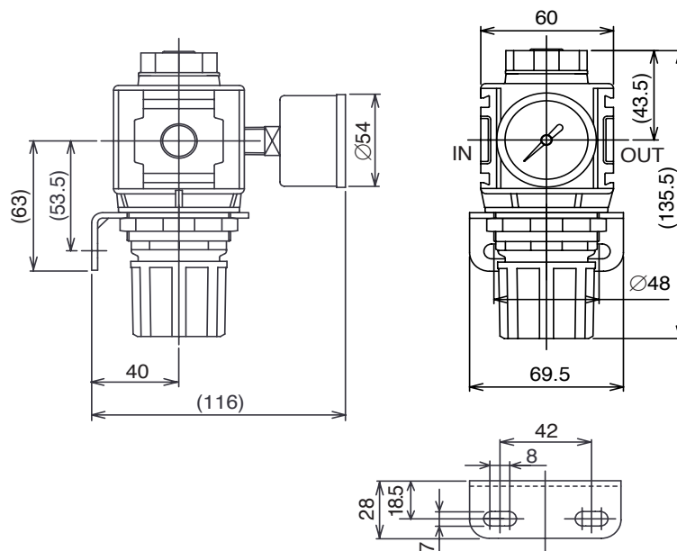
Bracket Mounting Dimensions
