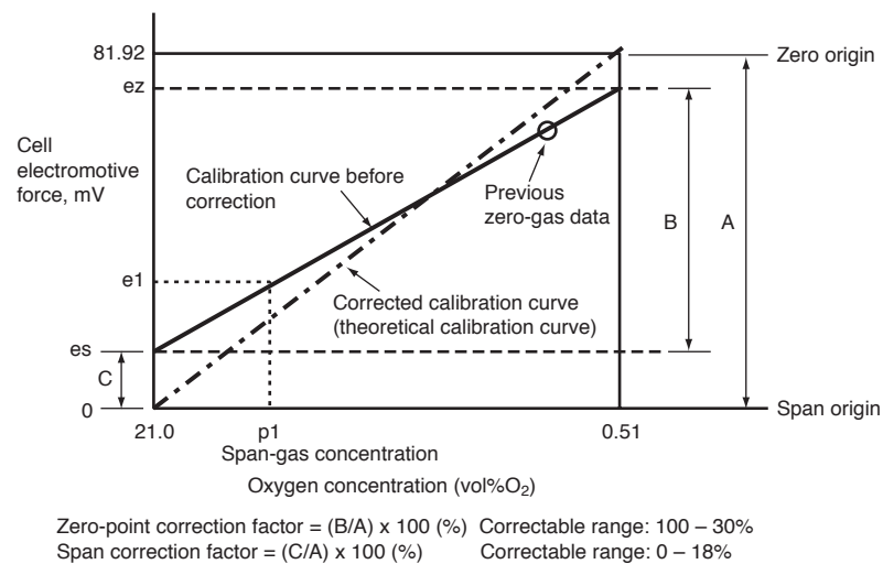
Figure 9.3 Calculation of a One-point Calibration Curve and Correction Factors using a Span Gas
