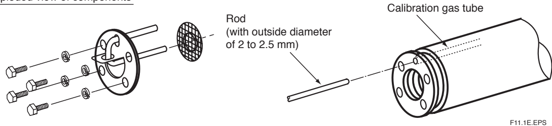
Figure 11.1 Cleaning the Calibration Gas Tube
