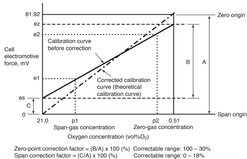
Figure 9.2 Calculation of a Two-point Calibration Curve and Correction Factors using Zero and Span Gases
