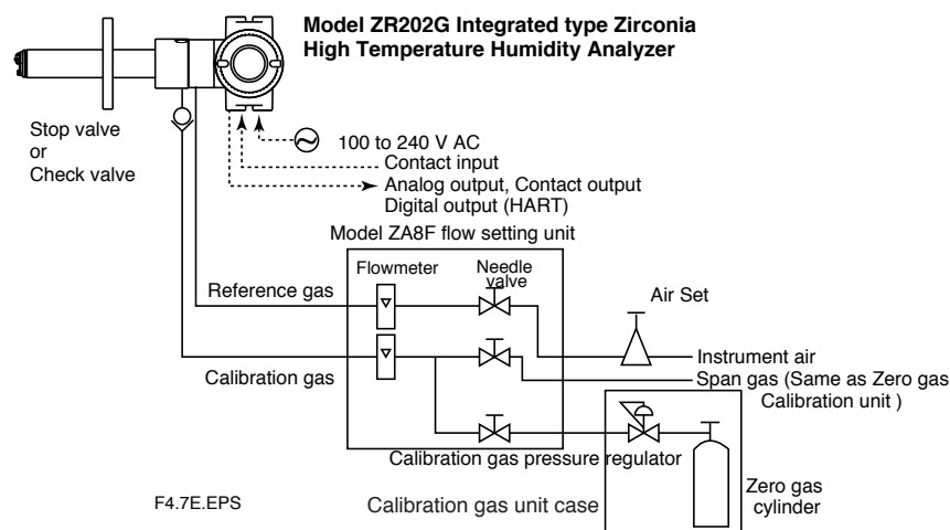
Figure 4.7 Piping for System 2
