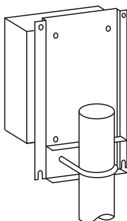
Figure 3.3 Pipe Mounting
