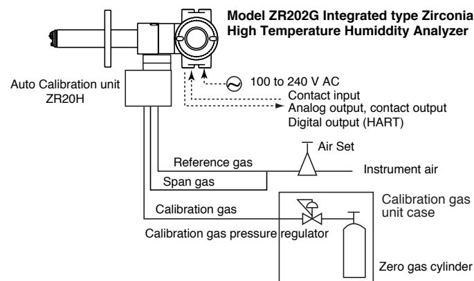
Figure 4.9 Piping for System 3
