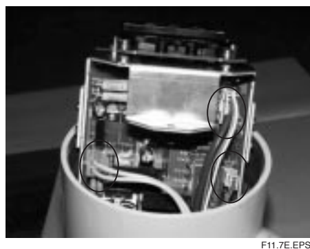
Figure 11.7 Locations of Connectors
