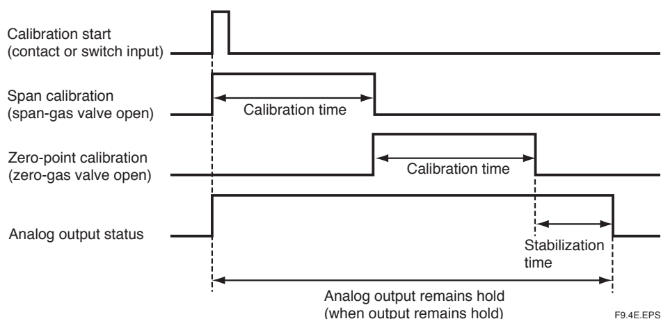
Figure 9.4 Calibration and Output-stabilization Time Settings
