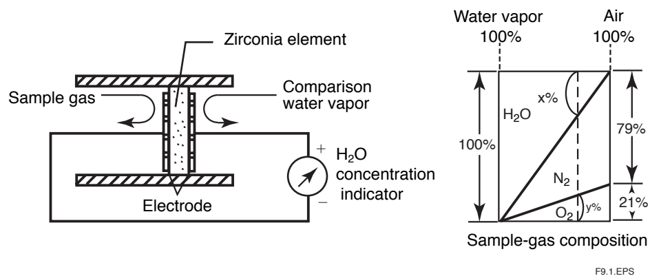
Figure 9.1 Schematic Diagram of Measurement Principle
