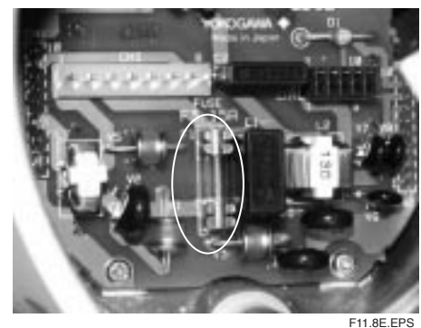
Figure 11.8 Location of Fuse
