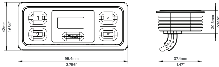
Fig. 6: Product dimensions, TOUCHinlay-KM
