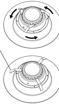
STEP 4 ALUMINUM TABS
