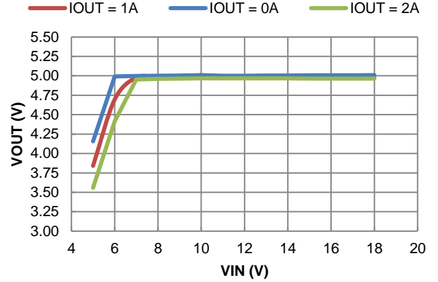
Figure 15. Line Regulation
