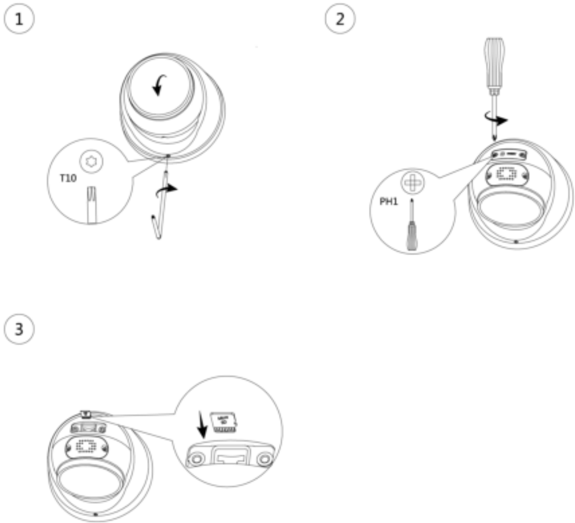
Figure 3-2 Installing SD card
