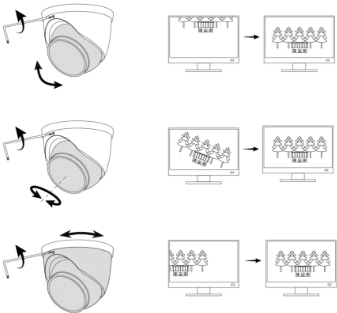
Figure 3-6 Adjusting lens angle
