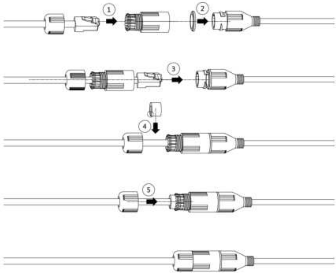
Figure 3-5 Installing waterproof connector
