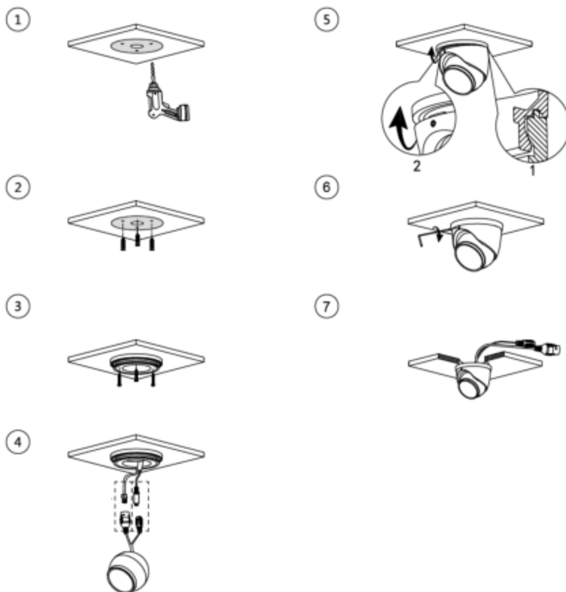
Figure 3-4 Cable going through the mounting surface
