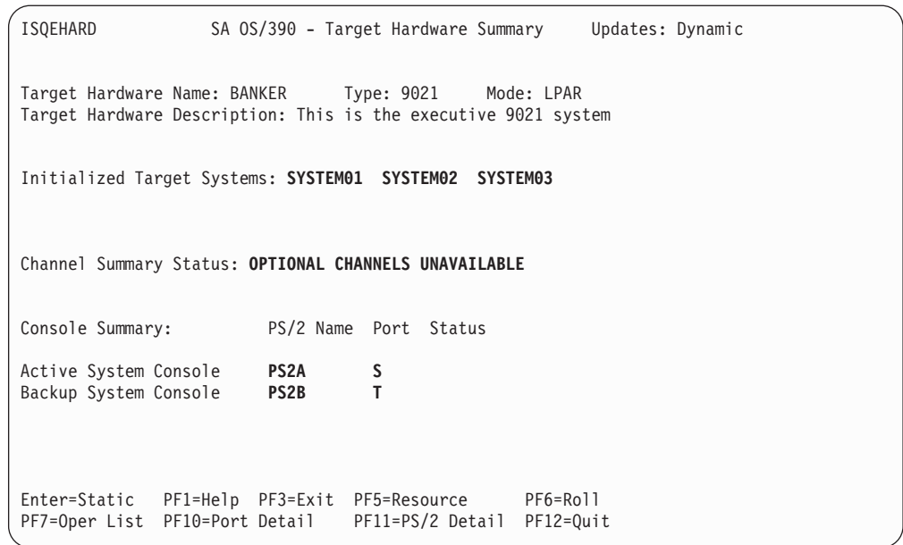
Figure 38. Target Hardware Summary Panel for Screen-Oriented Processor
