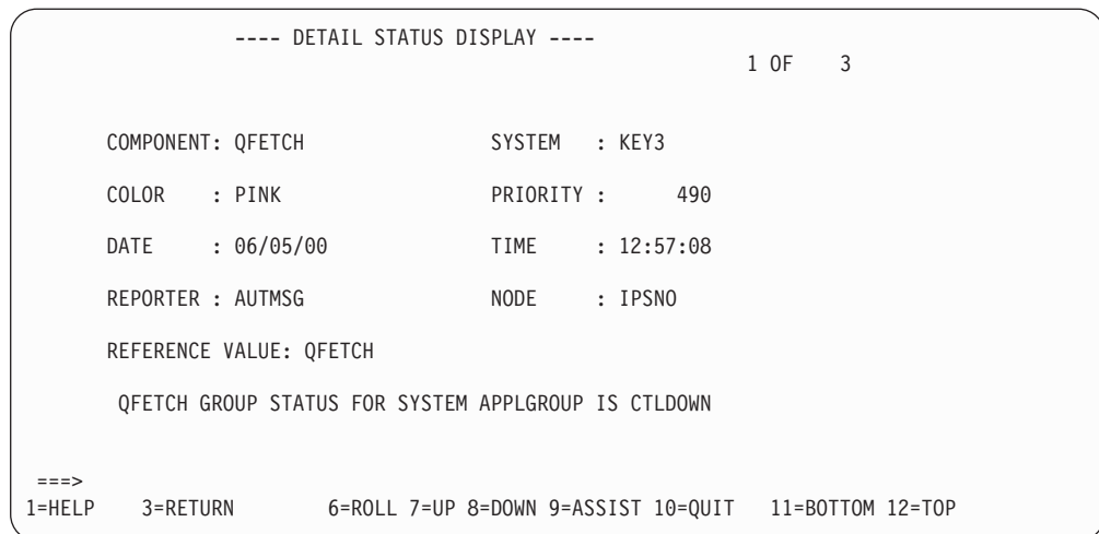
Figure 49. SDF Detail Status Display Panel for an Application group
