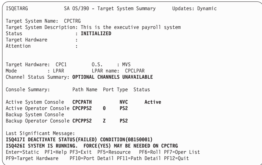
Figure 41. Target System Summary Panel
