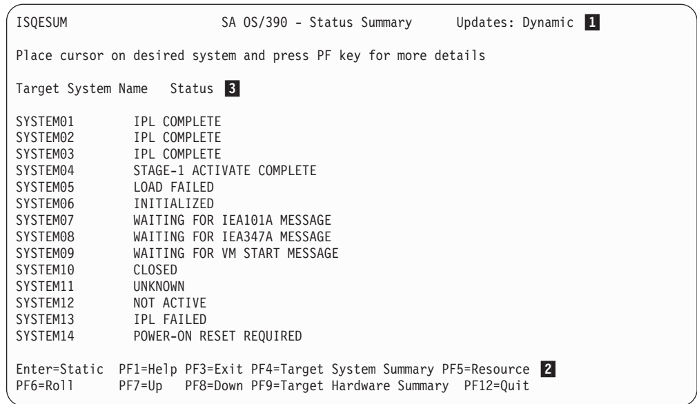
Figure 40. Status Summary Panel
