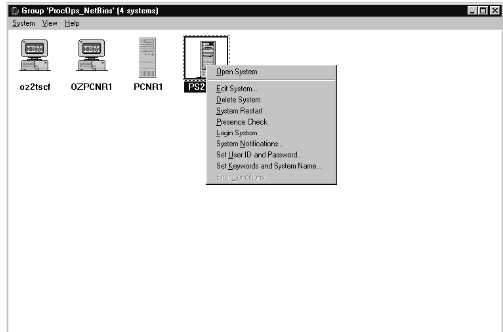
Figure 111. Group Window
