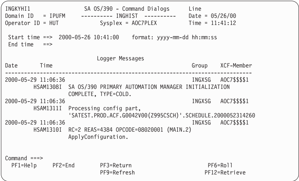
Figure 132. INGHIST Logger Messages
