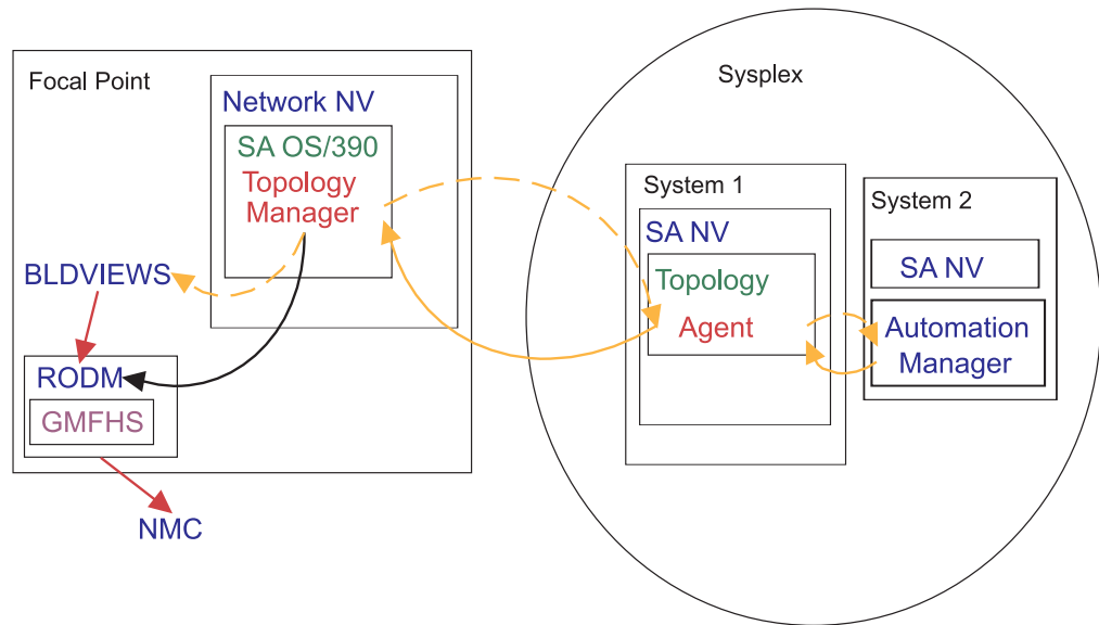
Figure 90. Topology Manager Overview
