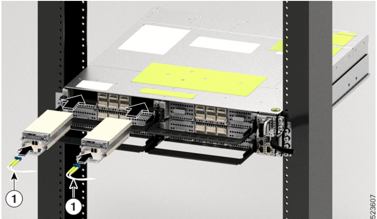
Figure 20: Inserting the CIM8 Module in 2.4T Card
