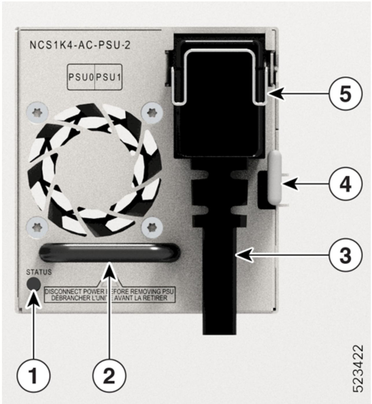
Figure 18: NCS1K4-AC-PSU-2 with 90-degree Cable Connection
