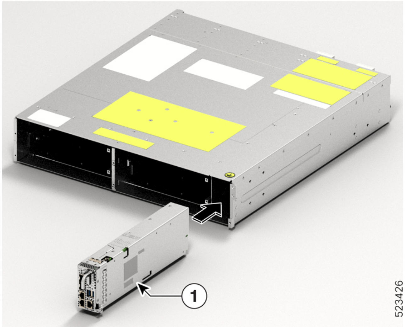
Figure 6: Inserting the Controller
