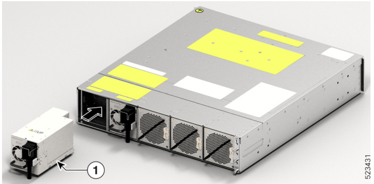
Figure 14: Inserting the PSU
