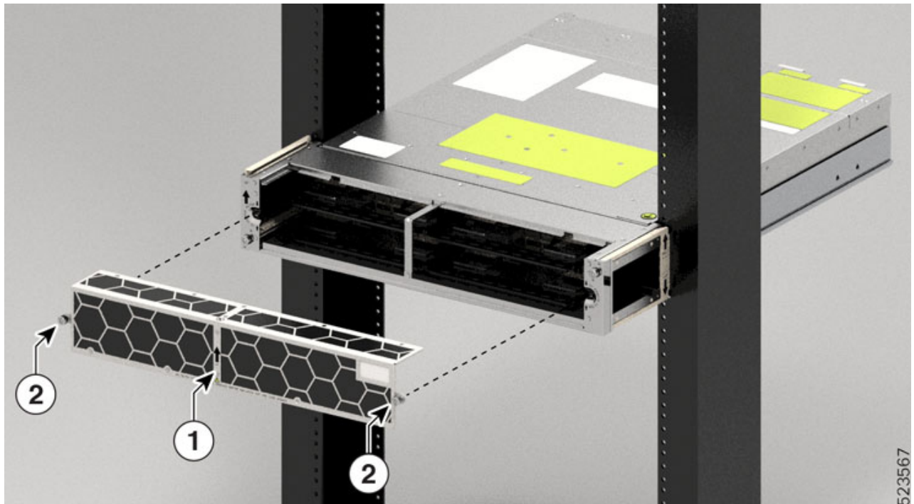
Figure 24: Installing the Air Filter
