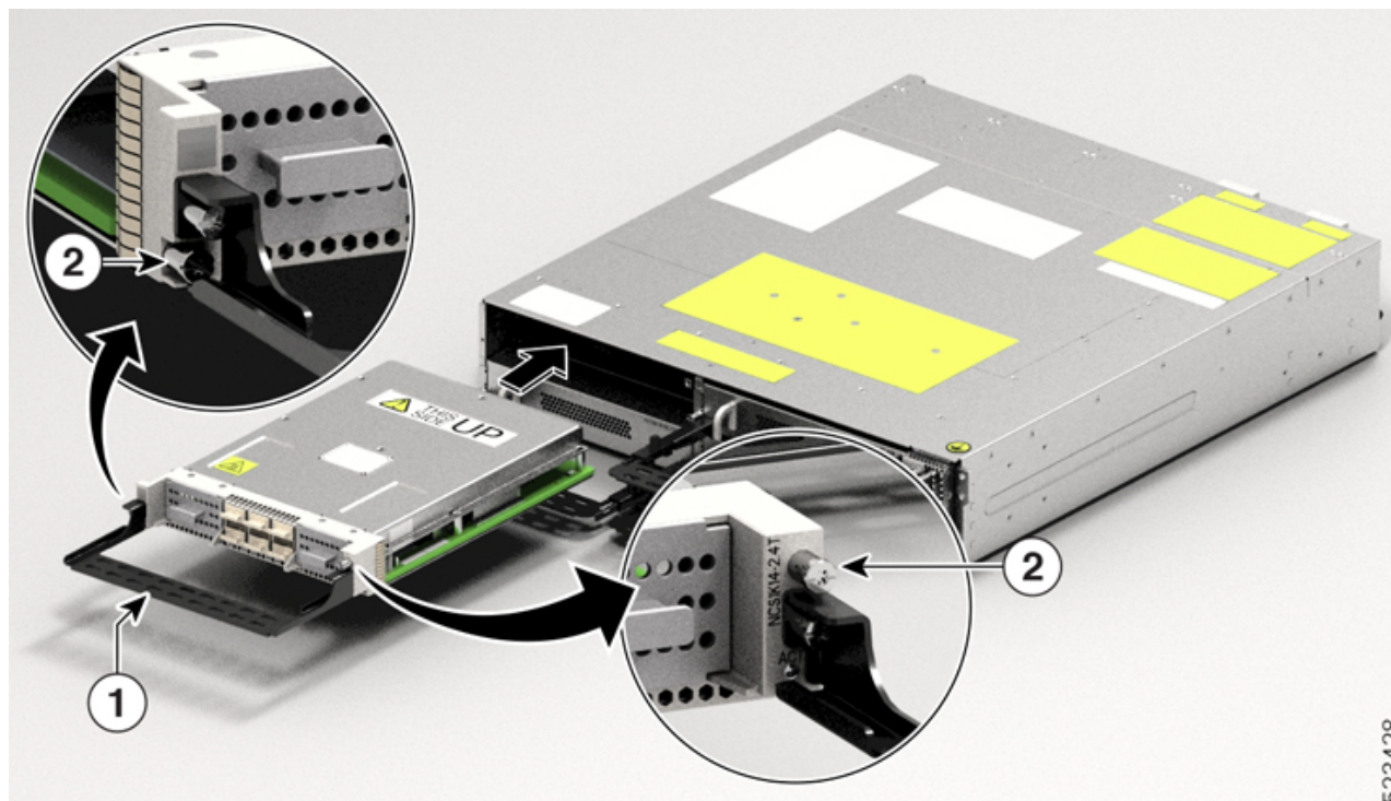
Figure 11: Inserting the NCS1K14-2.4T-K9 Line Card
