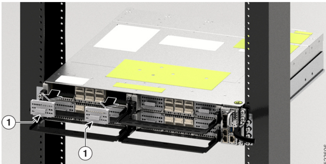
Figure 19: Removing the Dust Caps
