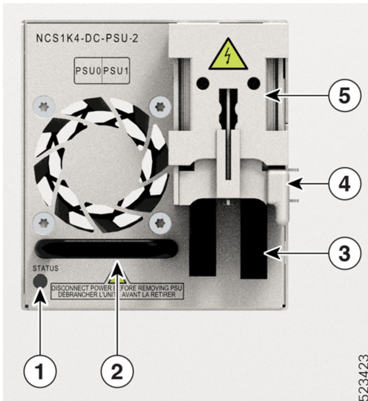
Figure 16: NCS1K4-DC-PSU-2 with 90-degree Cable Connection
