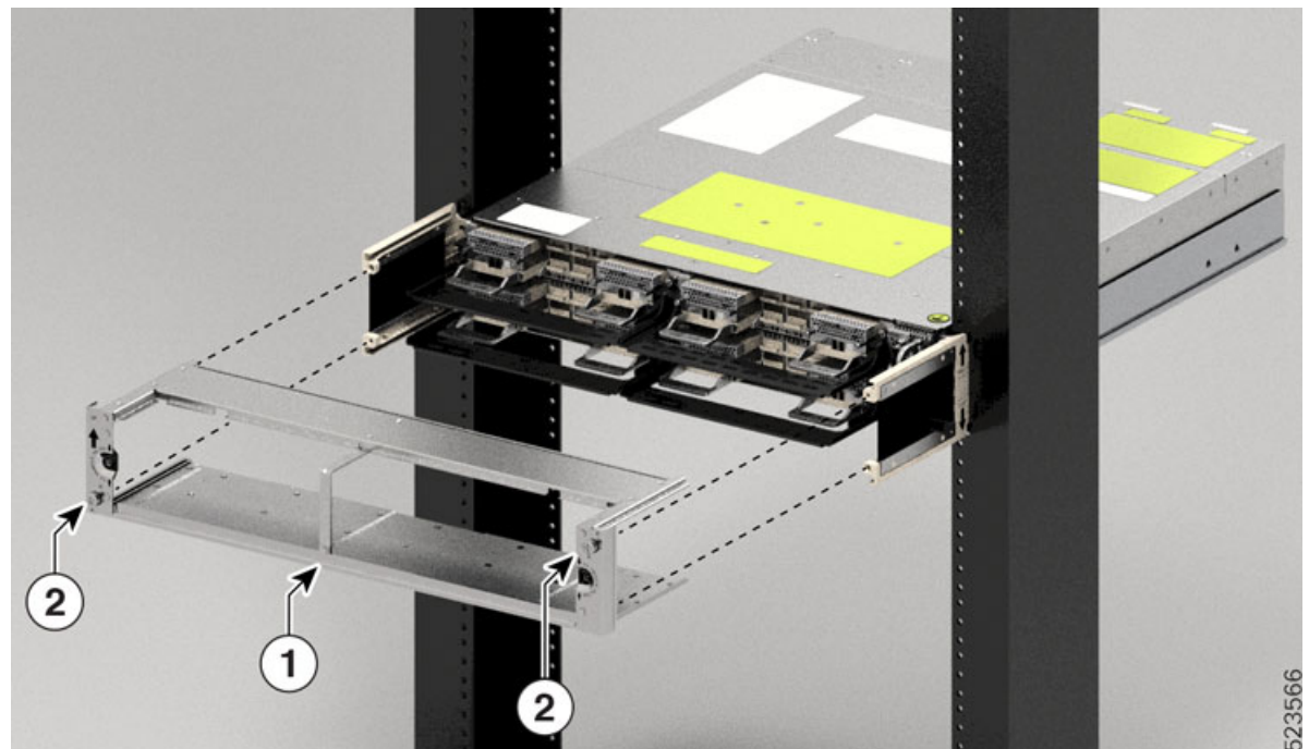
Figure 23: Installing the Air Filter Frame
