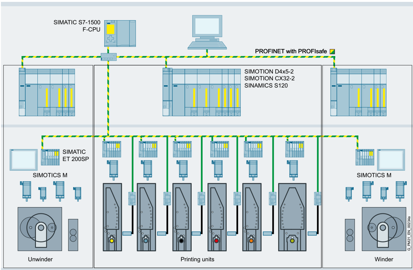
Example of gravure printing press with integrated TRC3000 register control
