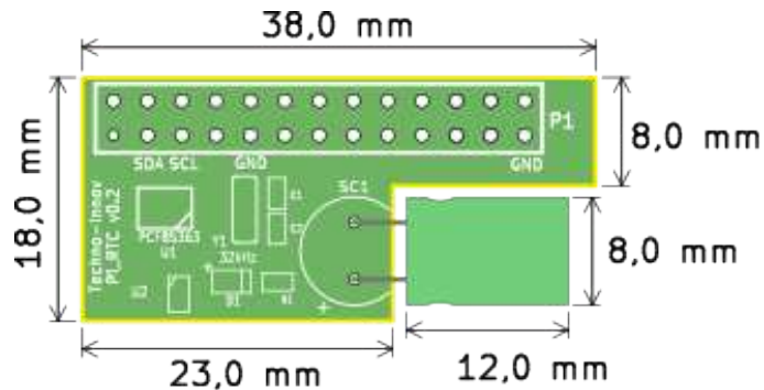
FIG 1 – Board dimensions
