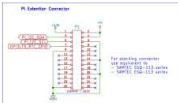
FIG 2 – P1 Connector
