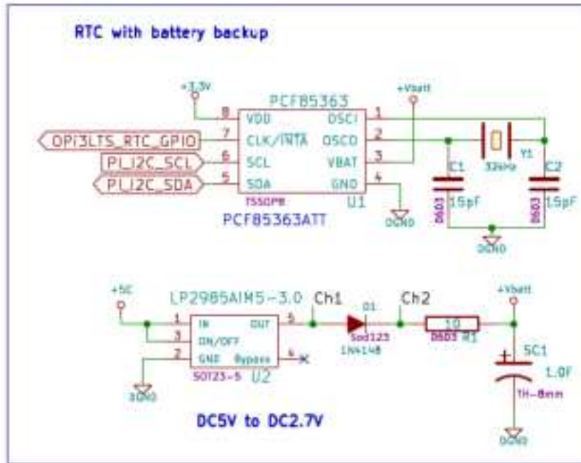
FIG 4 – RTC Clock
