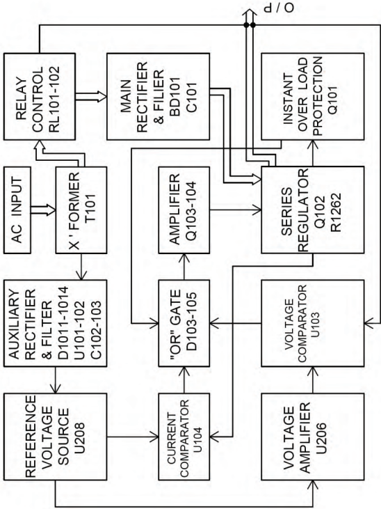
Block diagram
