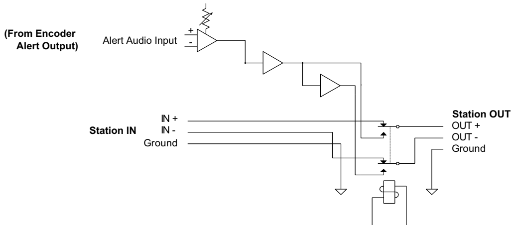
Figure 3. Typical relay showing in and out routing.
