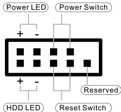
Motherboard Header Diagram
