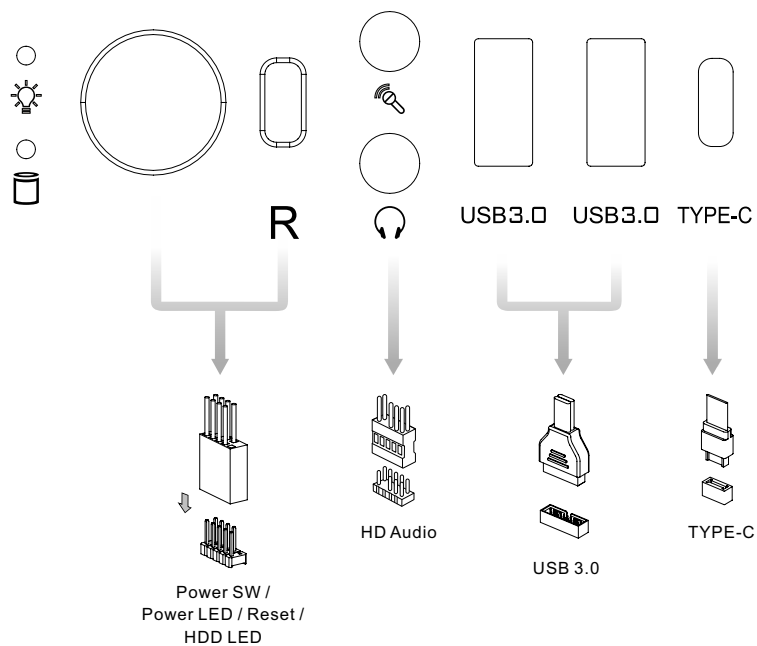
Motherboard Header Diagram
