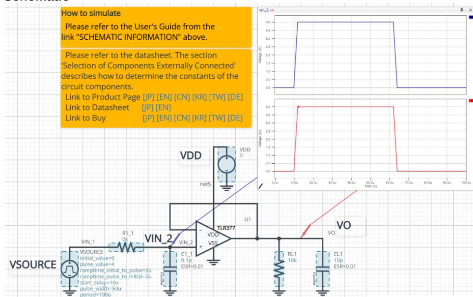
Figure 1. Simulation Schematic
