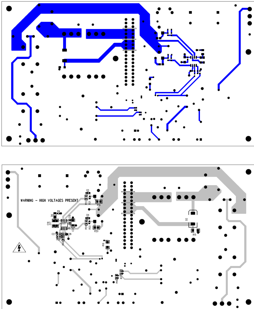
Figure 19. Motherboard PCB (Part 3/3)
