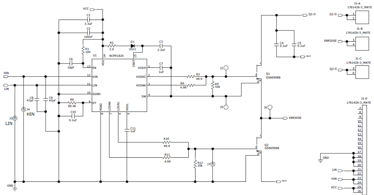
Figure 25. Daughter Card
