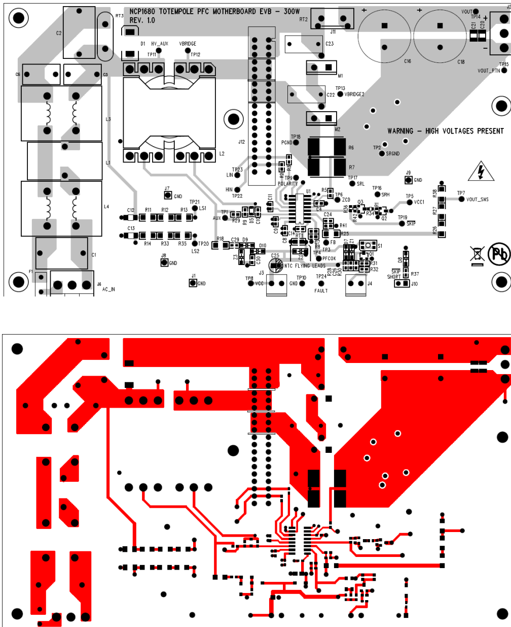
Figure 17. Motherboard PCB (Part 1/3)
