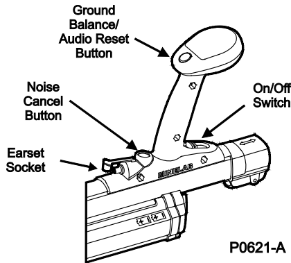
Figure 16: F3 Controls
