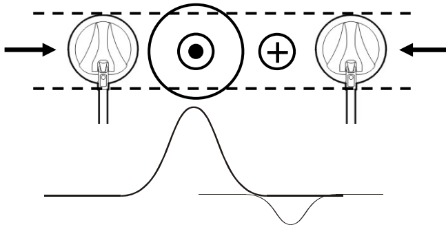
Figure 28: Multiple Targets
