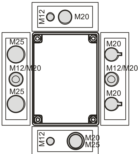
Fig. 4 Housing knockouts
