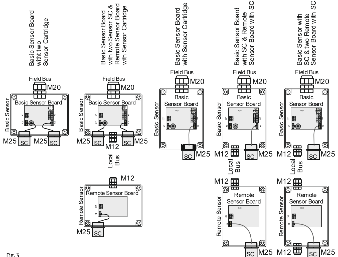
Fig. 3 Mounting possibilities
