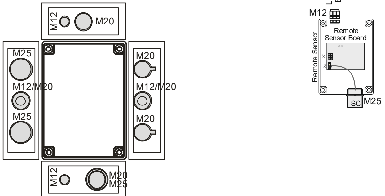
Fig. 4 Housing knockouts
