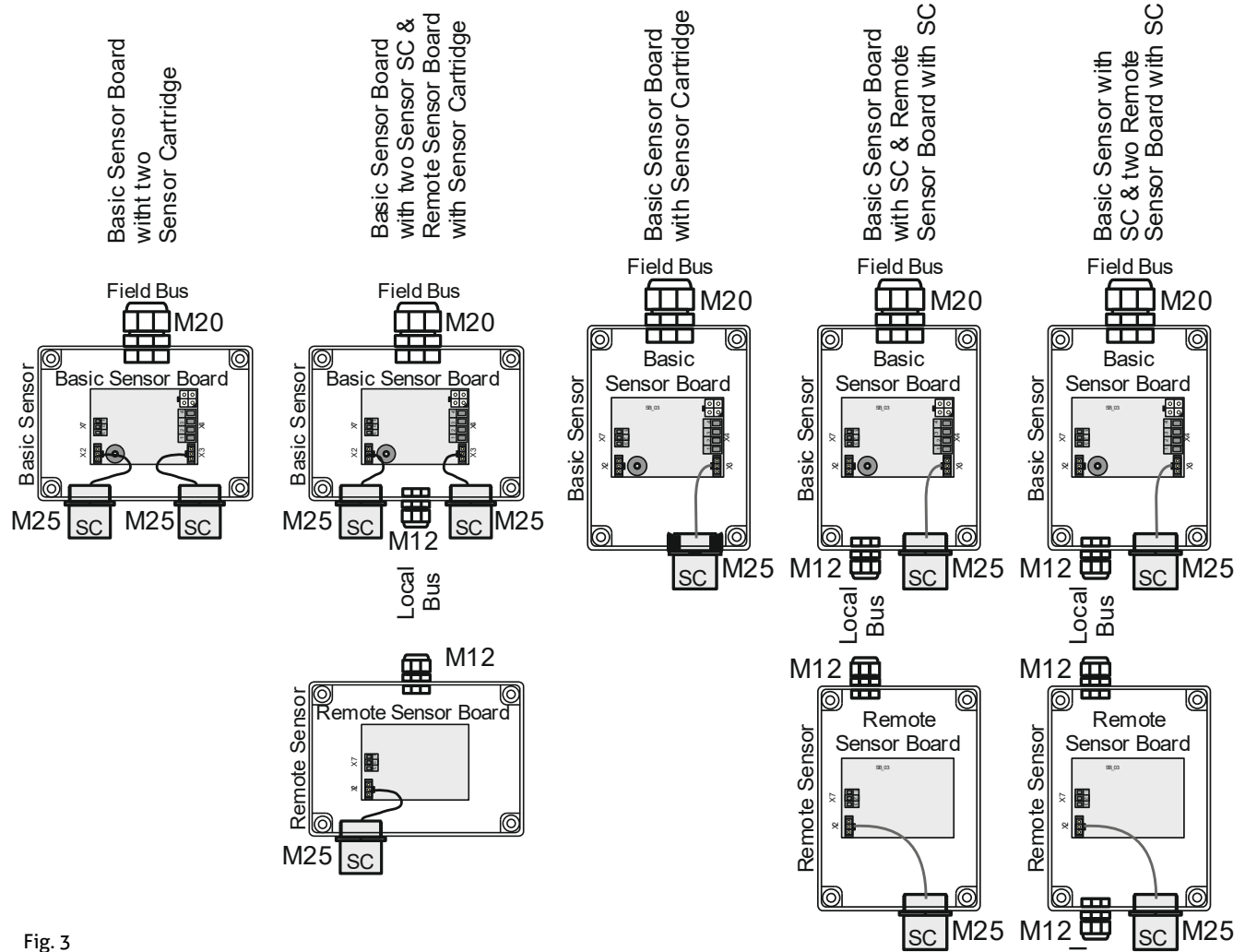
Fig. 3 Mounting possibilities
