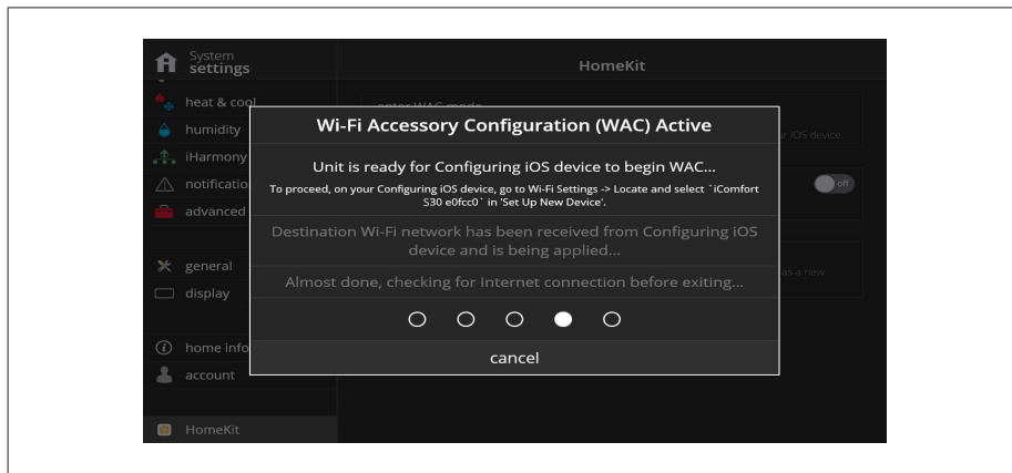
Figure 24. Wi-Fi Configuration
