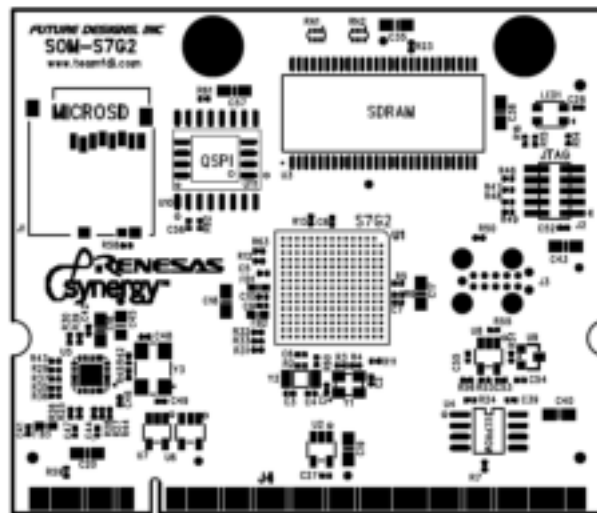
Figure 7: S7G2 Top
