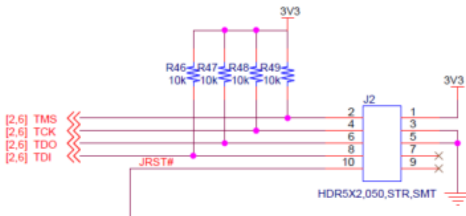
Figure 6: Tag-Connect JTAG
