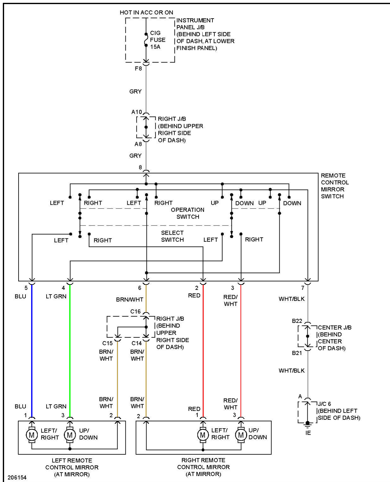
Fig. 32: Power Mirror Circuit
