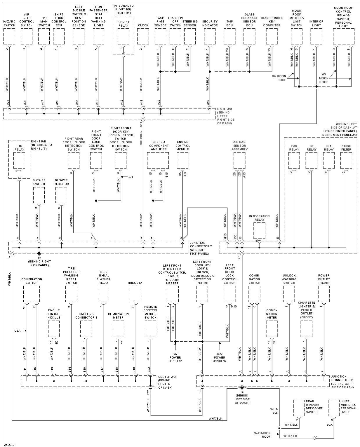
Fig. 20: Ground Distribution Circuit (1 of 2)
