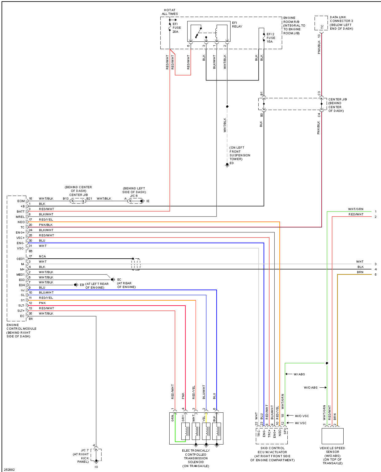
Fig. 43: A/T Circuit (1 of 2)
