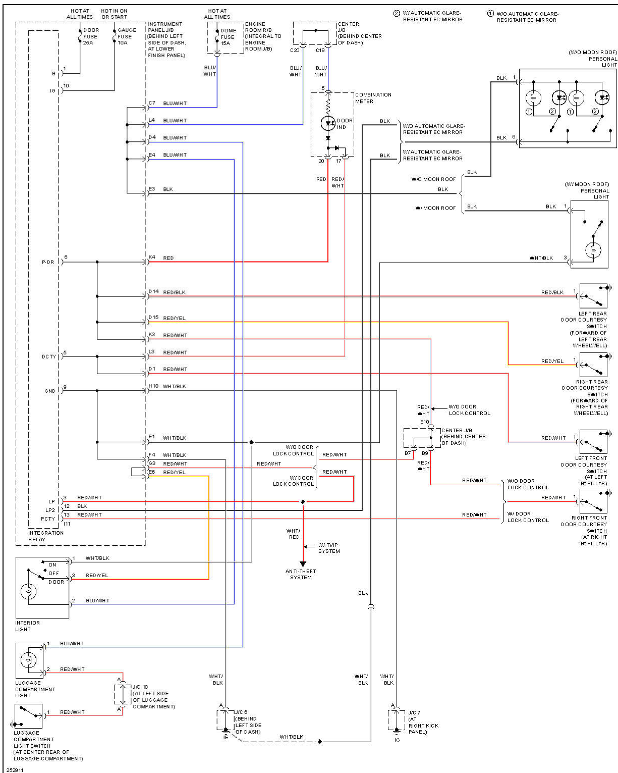
Fig. 25: Courtesy Lamps Circuit
