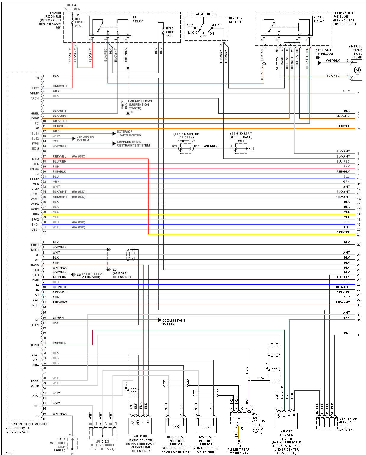
Fig. 14: 1.8L, Engine Performance Circuit (1 of 4)
