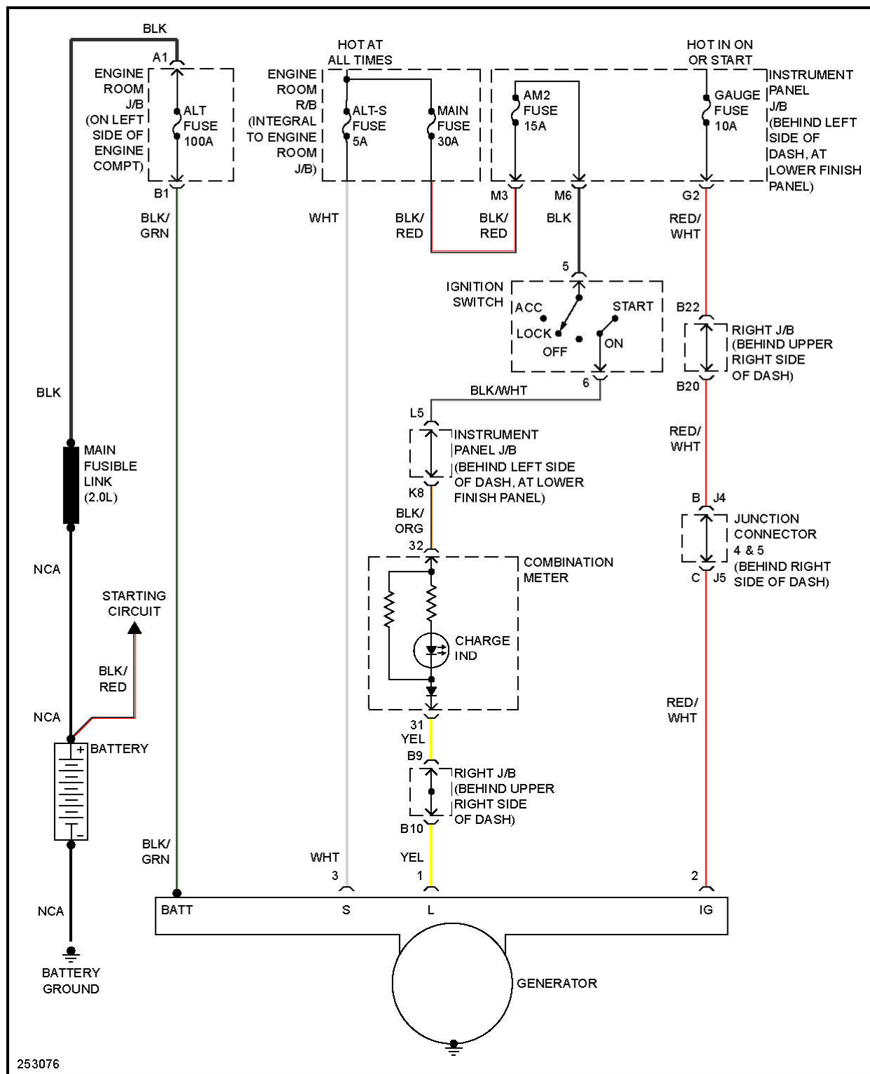
Fig. 38: Charging Circuit
