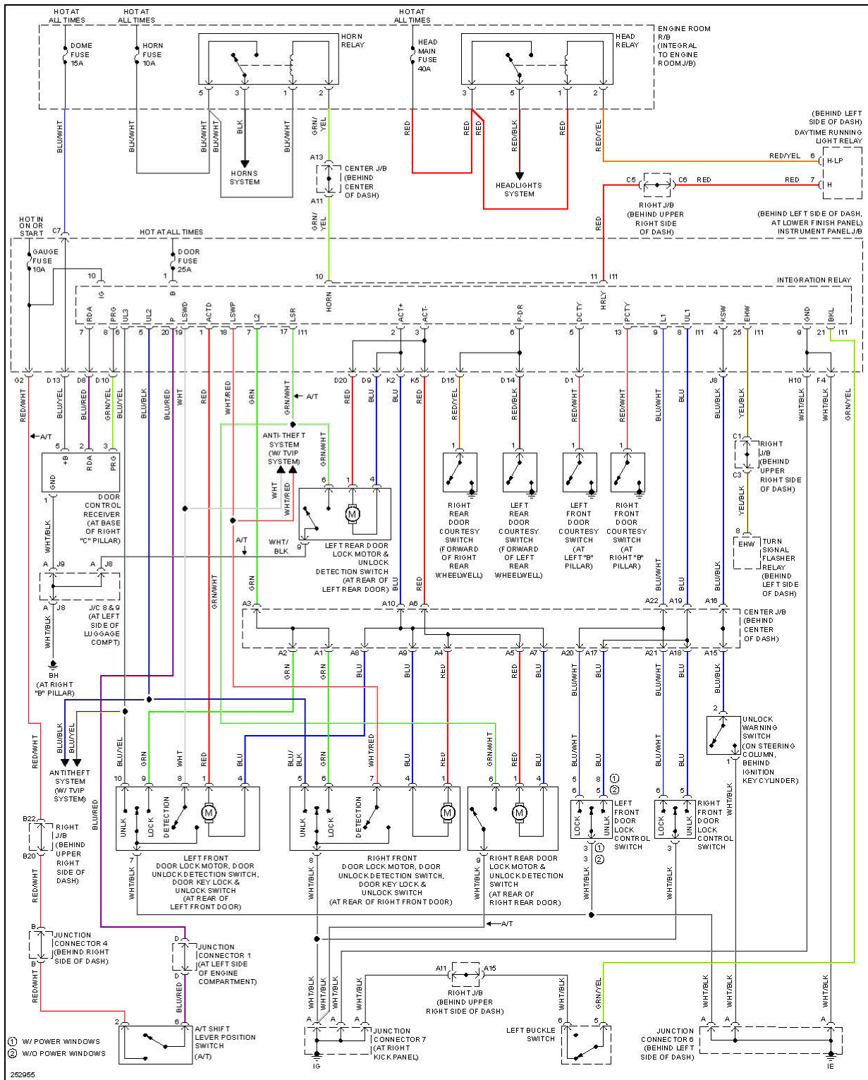
Fig. 29: Power Door Locks Circuit, W/ Keyless Entry
