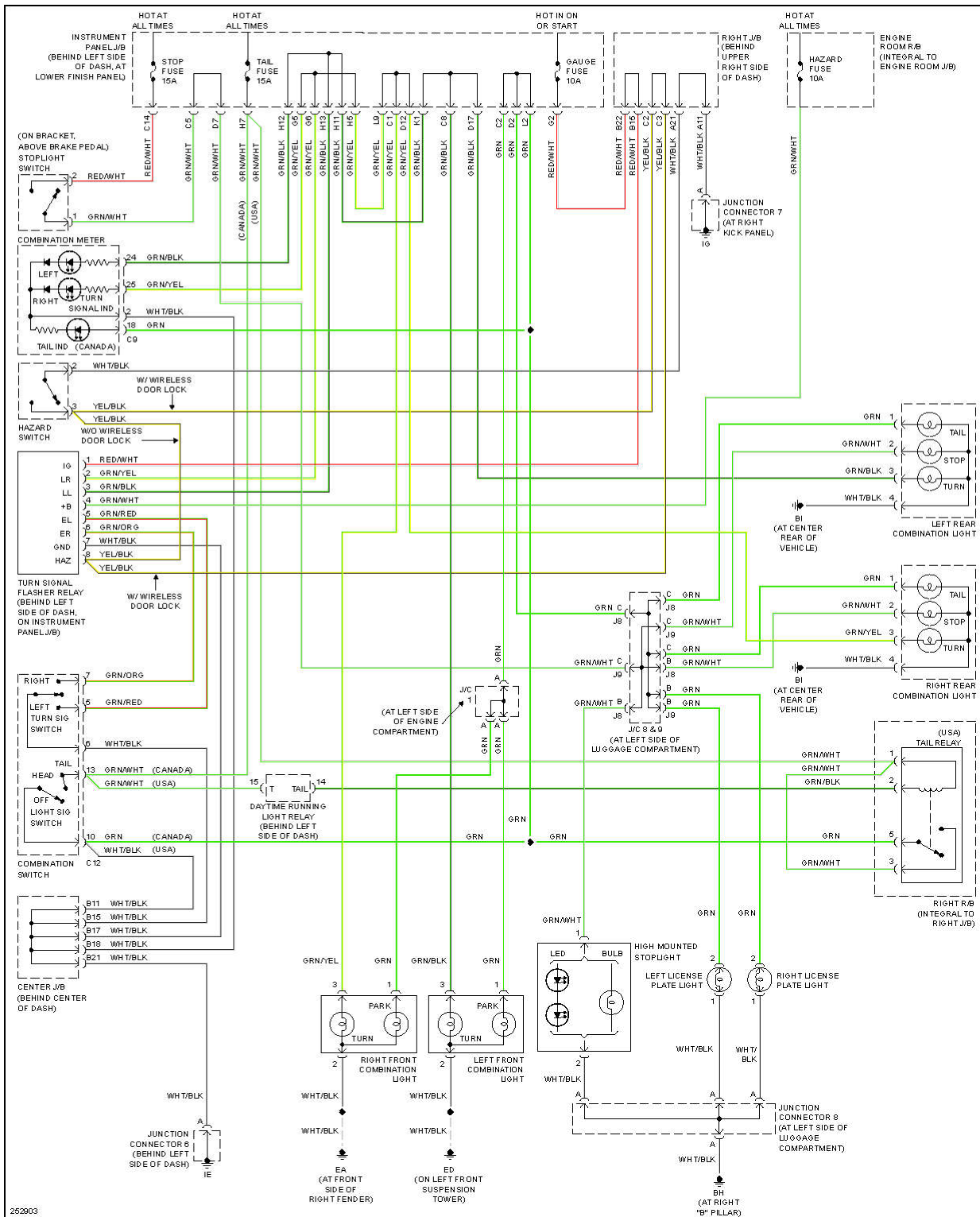
Fig. 19: Exterior Lamps Circuit
