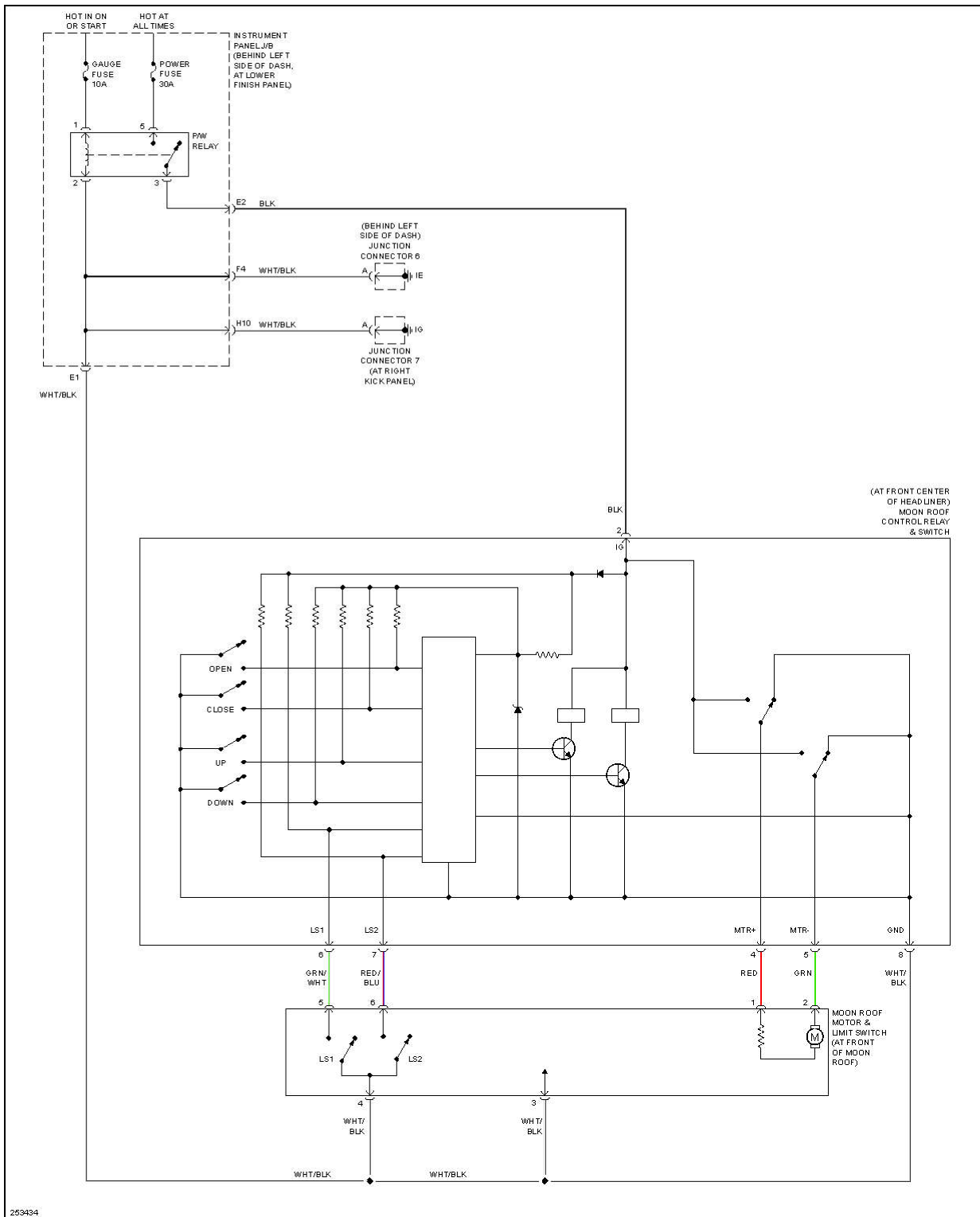
Fig. 33: Power Top/Sunroof Circuit
