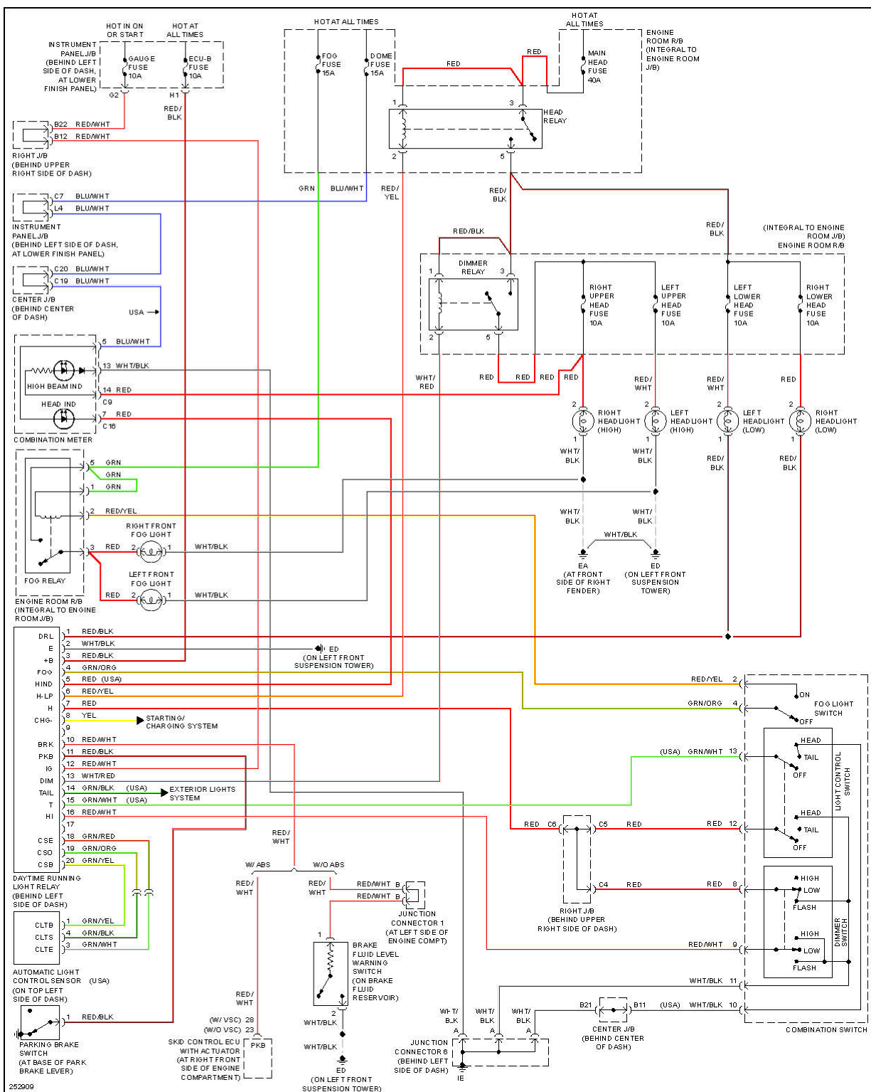
Fig. 22: Headlights Circuit
