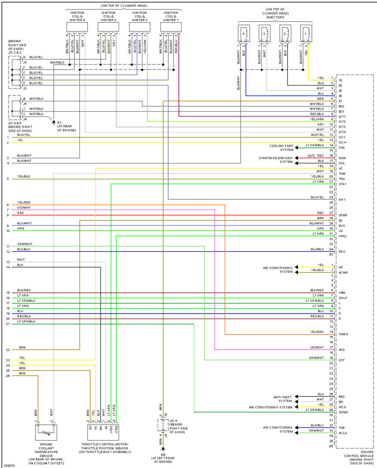
Fig. 17: 1.8L, Engine Performance Circuit (4 of 4)
