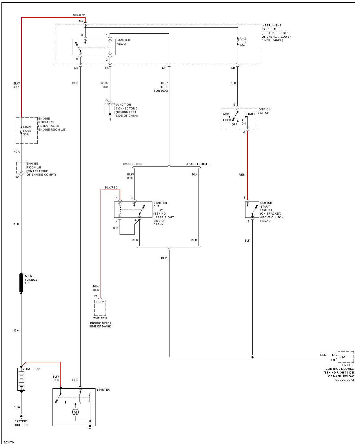
Fig. 40: Starting Circuit, M/T
