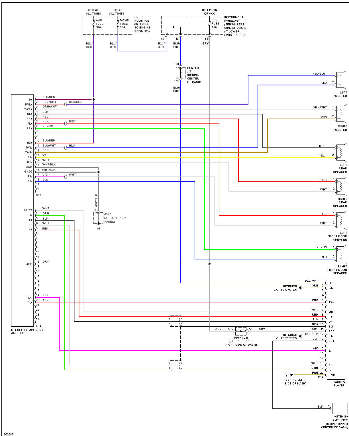
Fig. 35: Radio Circuit, W/ Amplifier
