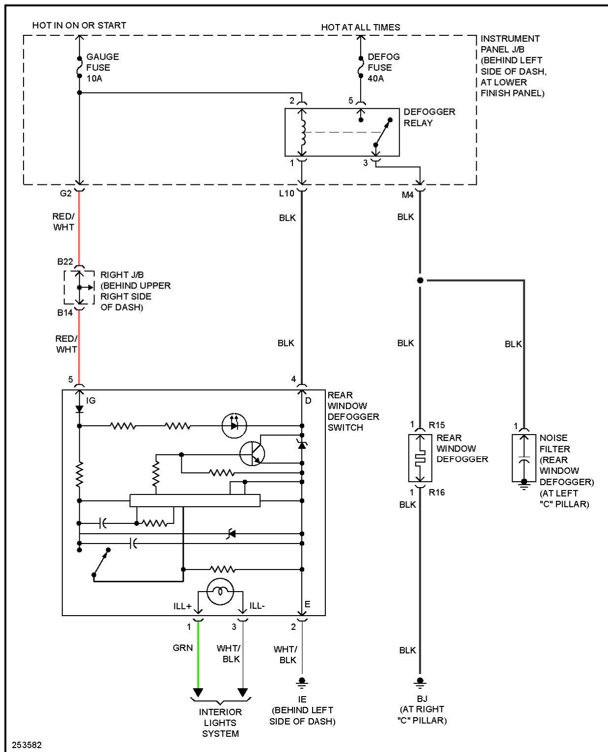
Fig. 13: Defoggers Circuit
