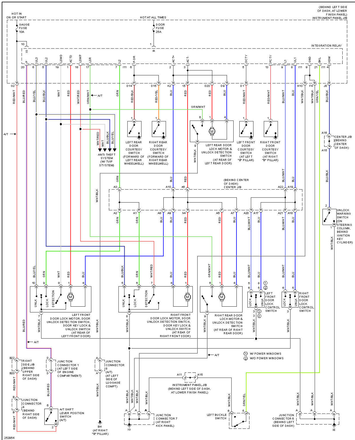
Fig. 30: Power Door Locks Circuit, W/O Keyless Entry
