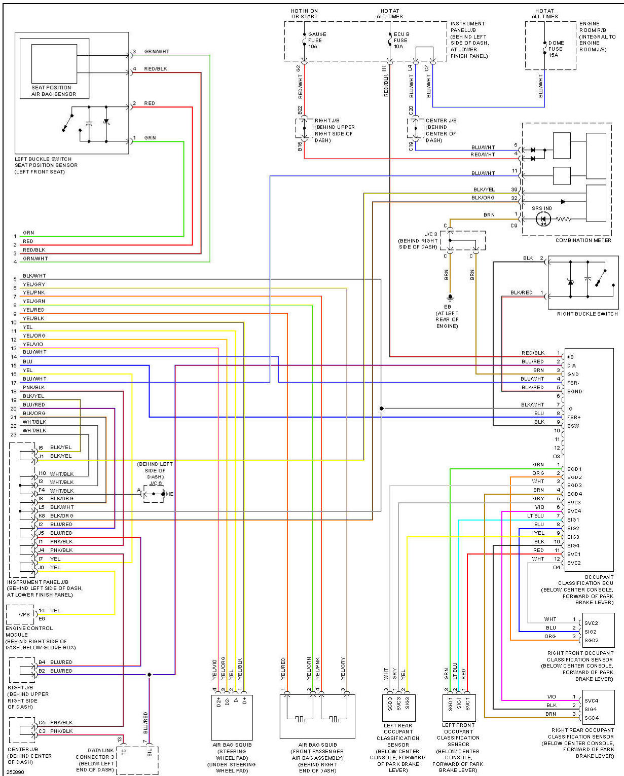
Fig. 42: Supplemental Restraints Circuit (2 of 2)
