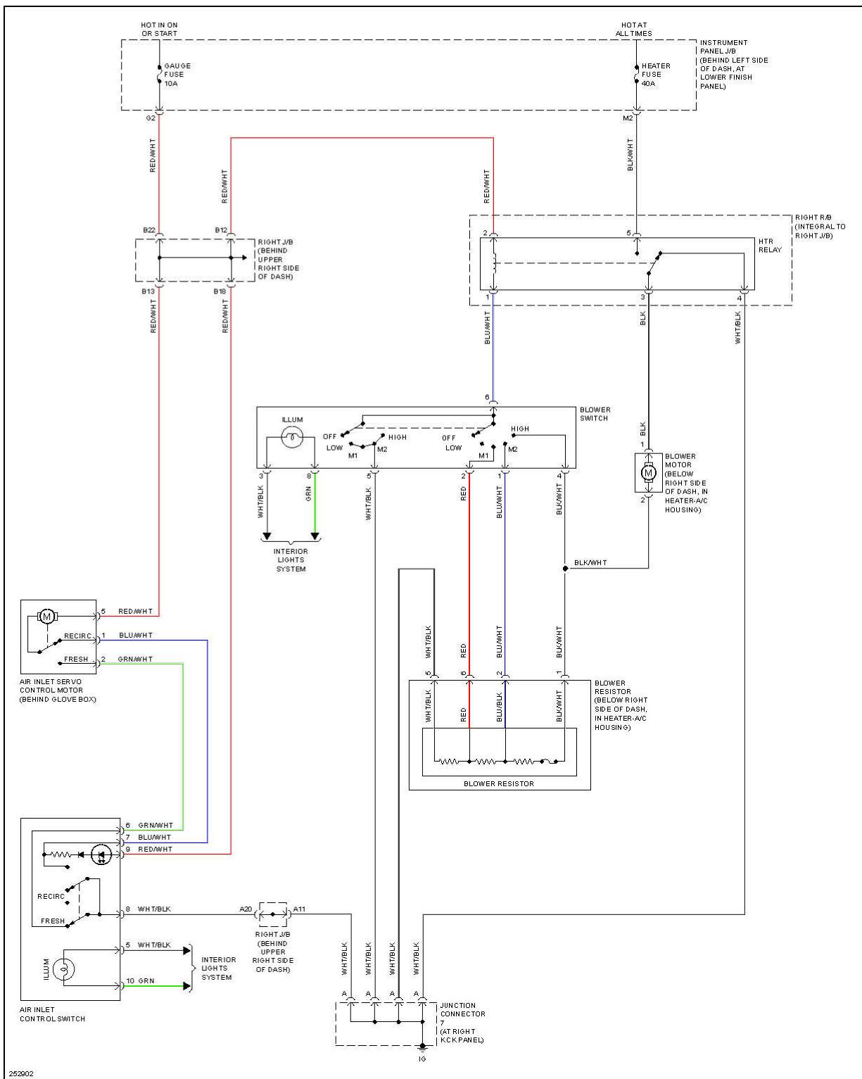
Fig. 1: Heater Circuit
