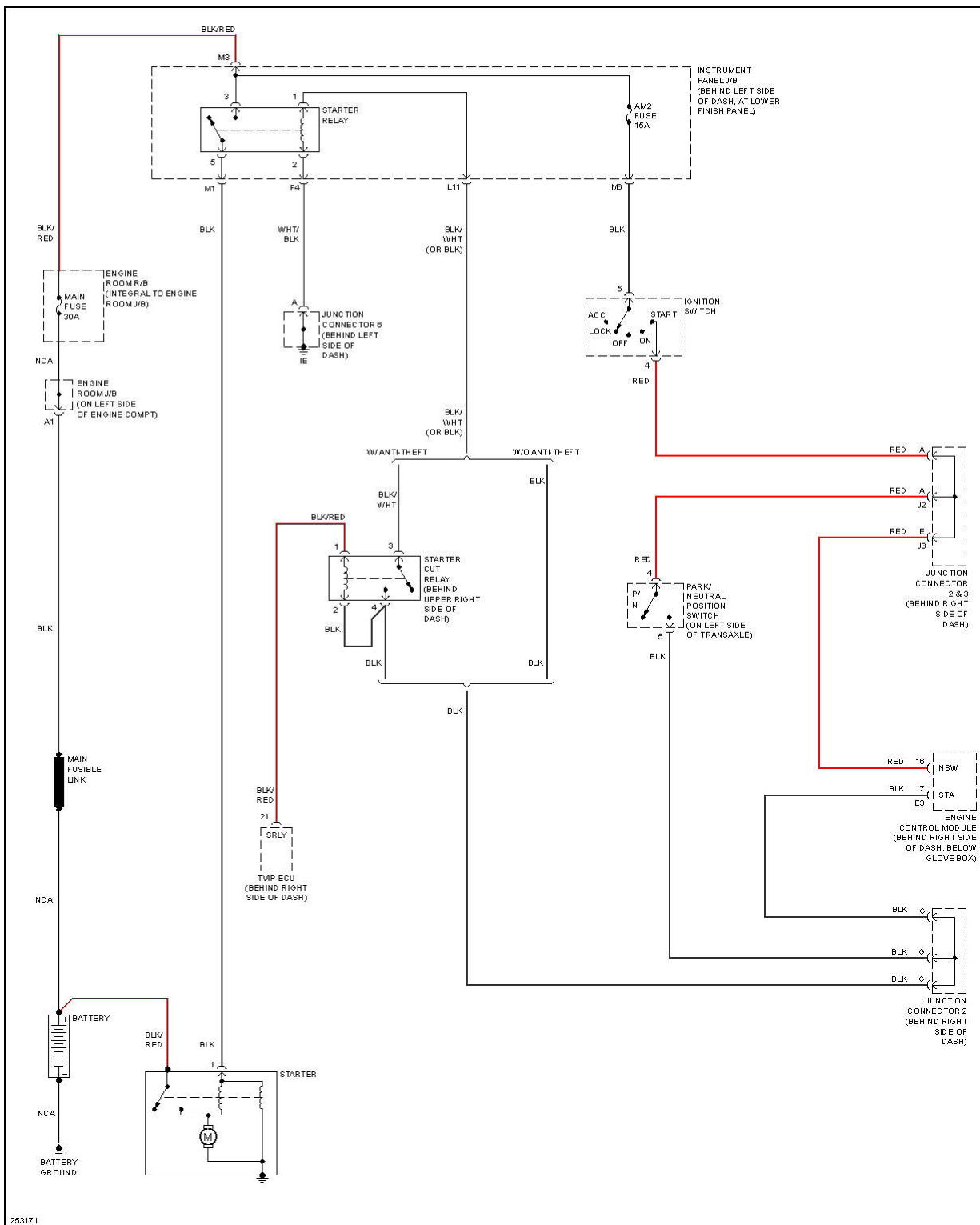
Fig. 39: Starting Circuit, A/T
