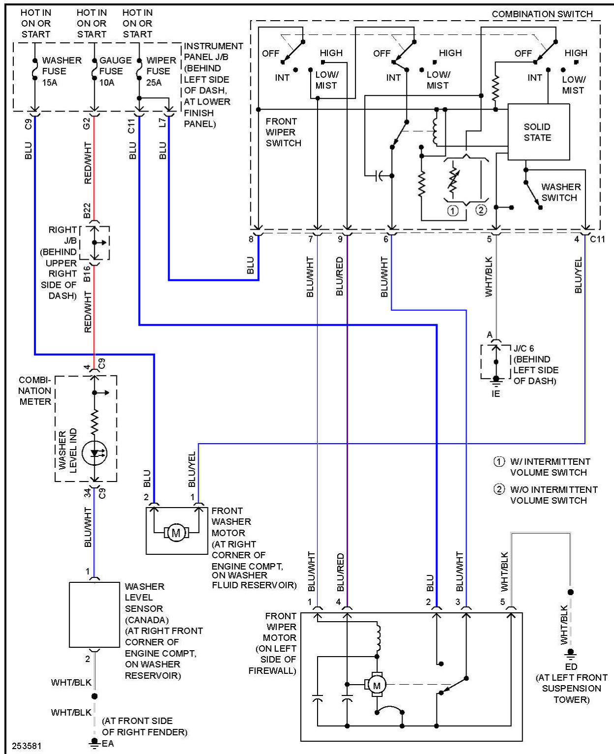
Fig. 48: Wiper/Washer Circuit
