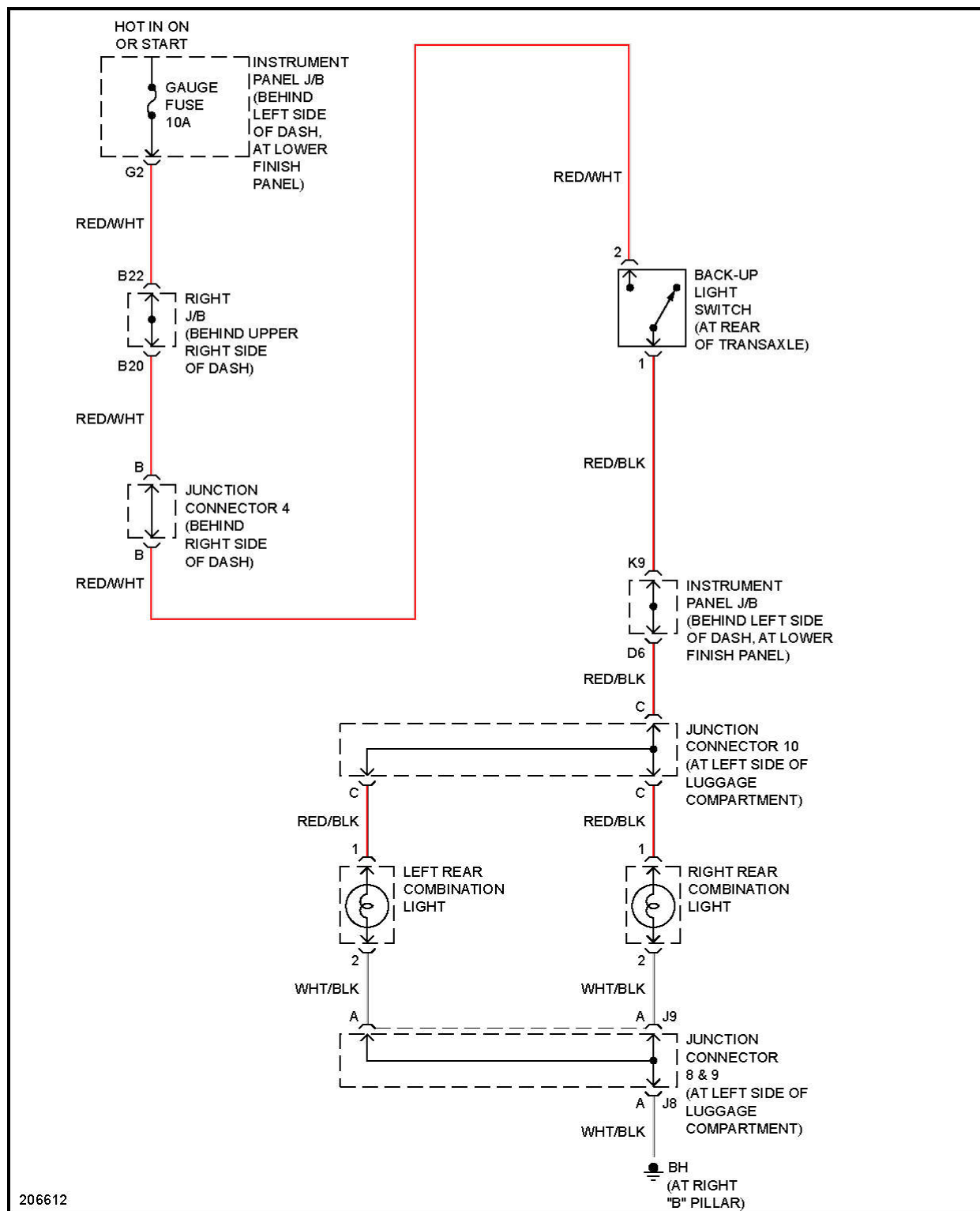
Fig. 18: Back-up Lamps Circuit
