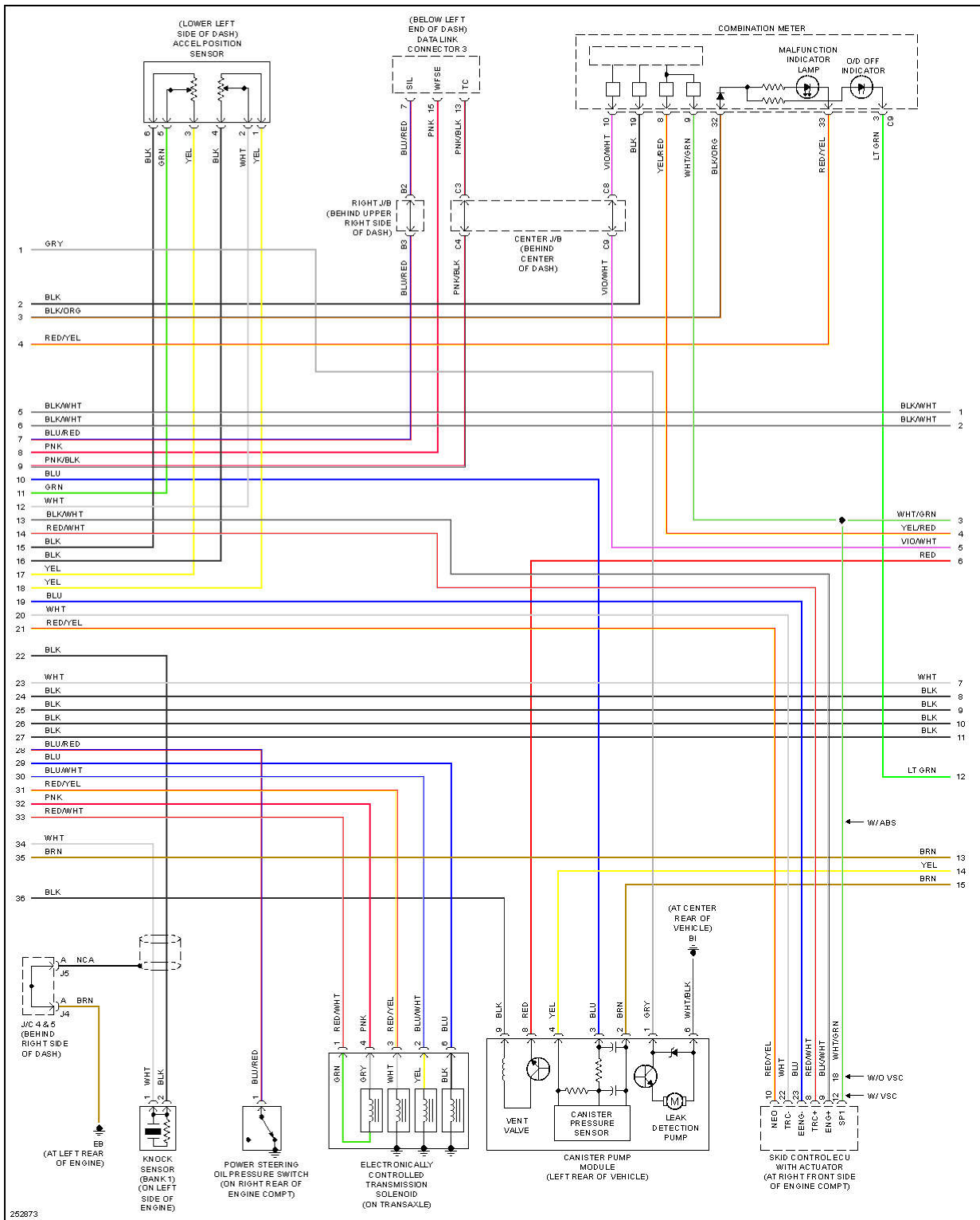
Fig. 15: 1.8L, Engine Performance Circuit (2 of 4)
