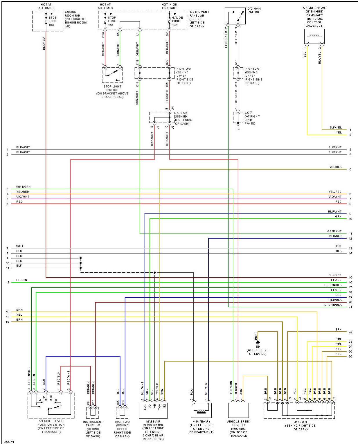
Fig. 16: 1.8L, Engine Performance Circuit (3 of 4)
