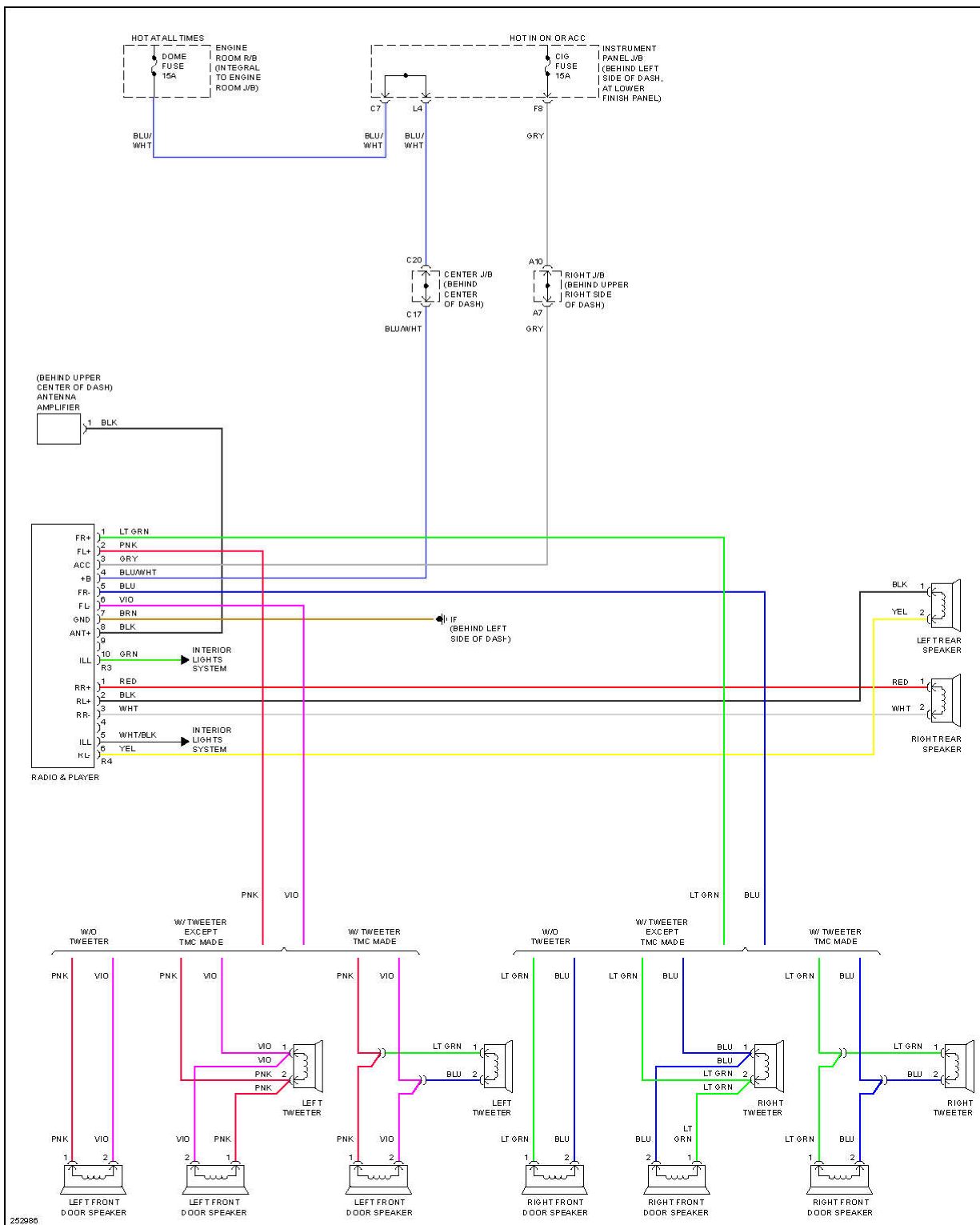
Fig. 36: Radio Circuit, W/O Amplifier
