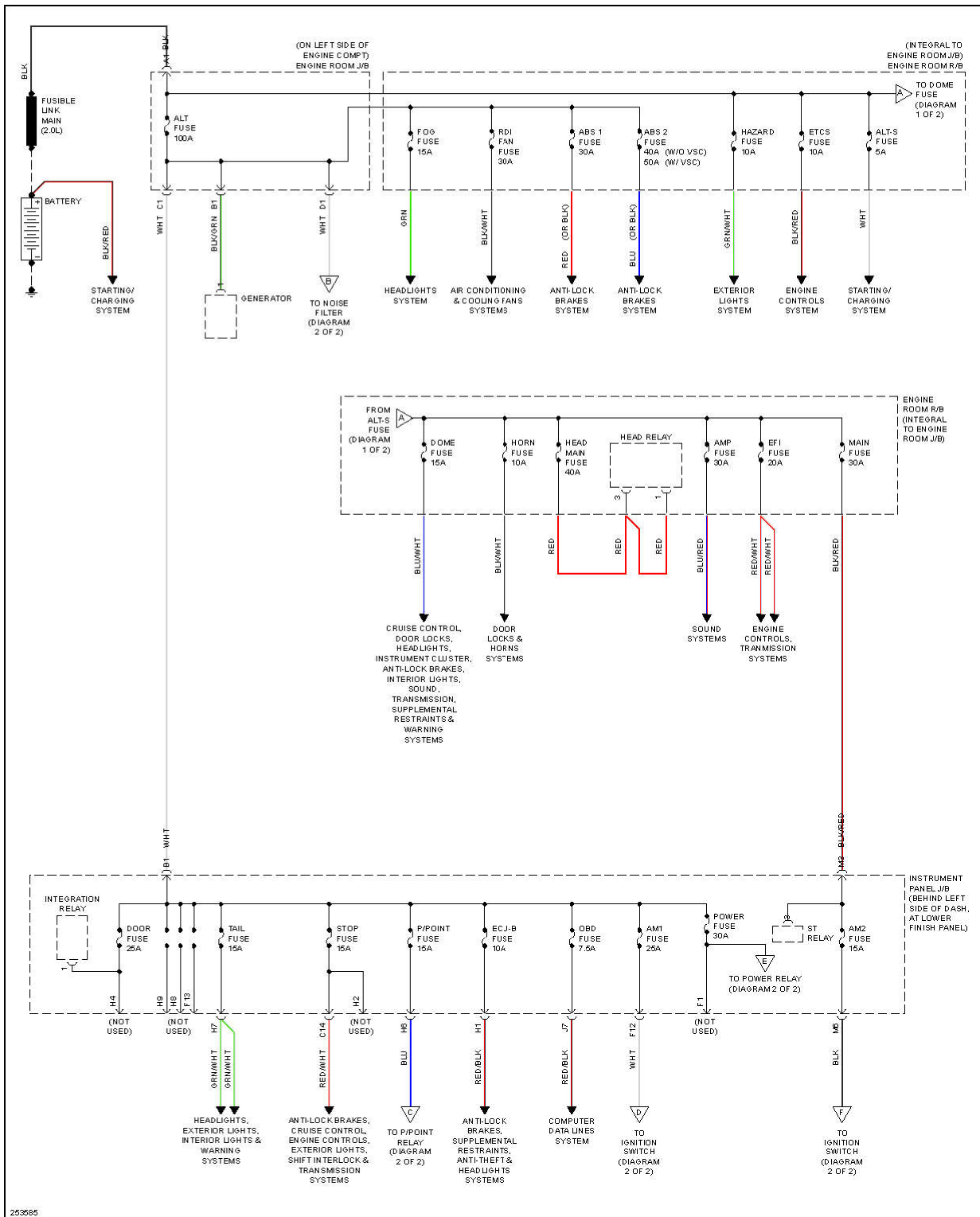
Fig. 27: Power Distribution Circuit (1 of 2)
