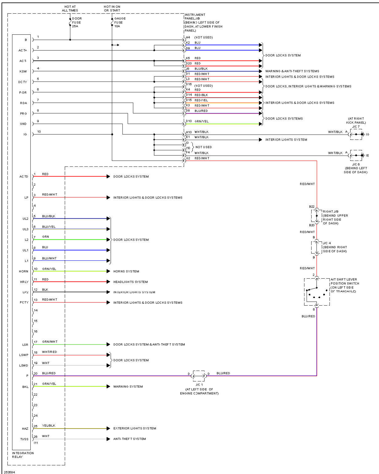
Fig. 9: Body Control Modules Circuit
