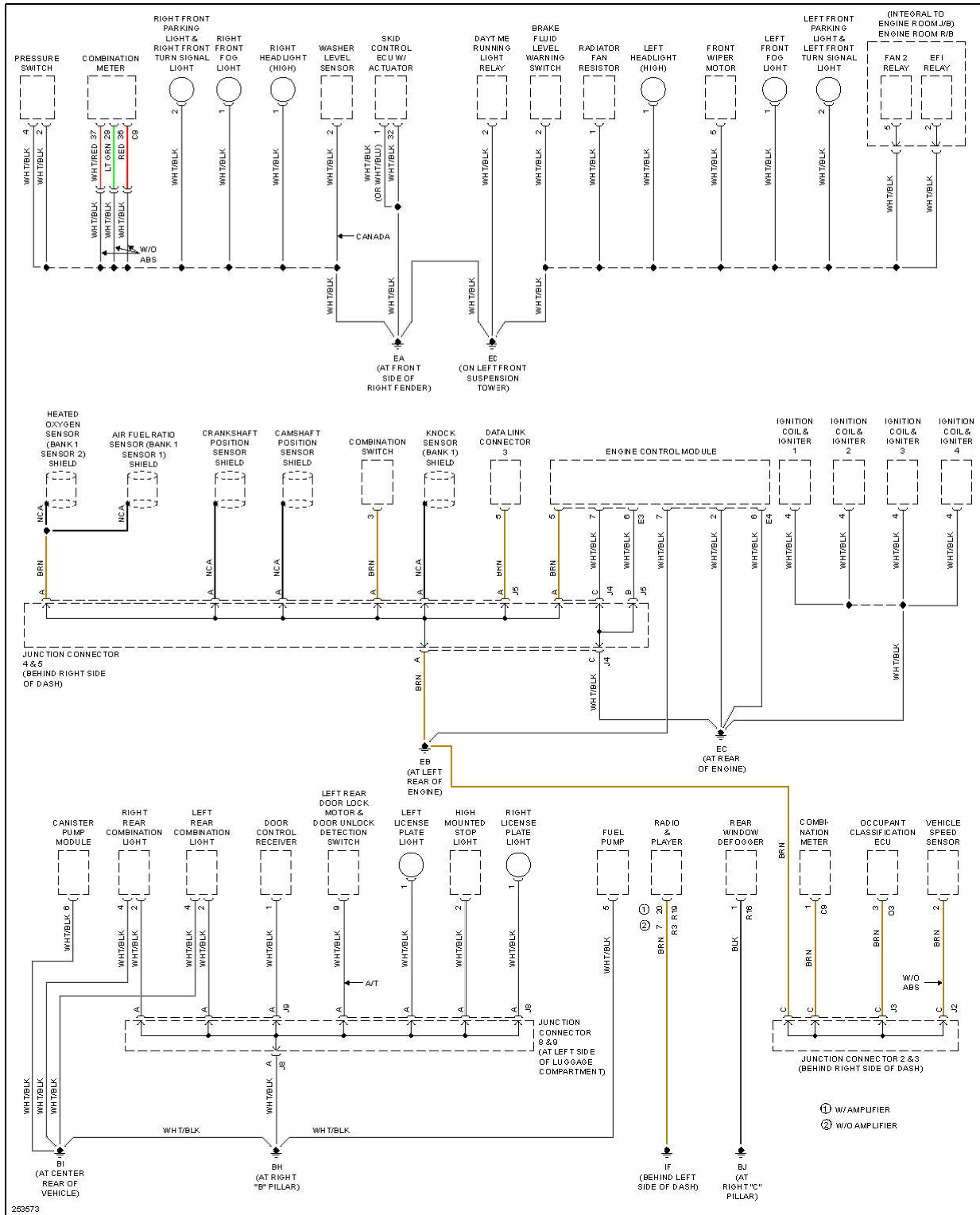
Fig. 21: Ground Distribution Circuit (2 of 2)
