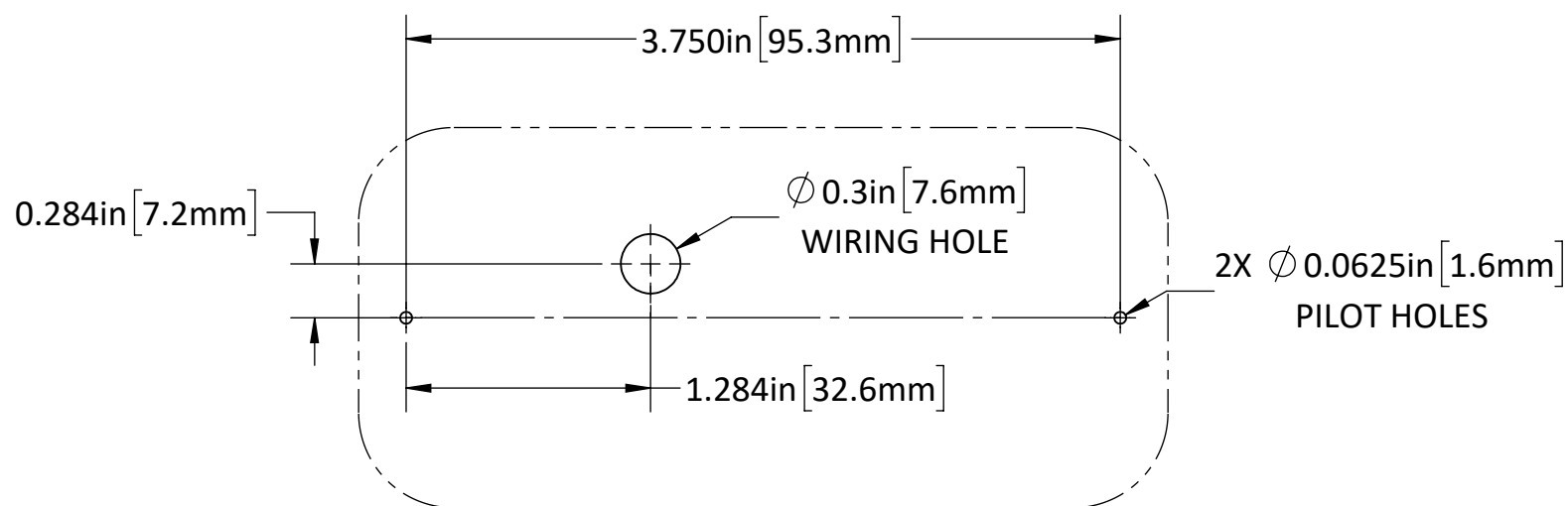
MOUNTING TEMPLATE PRINT AT 1:1 SCALE
