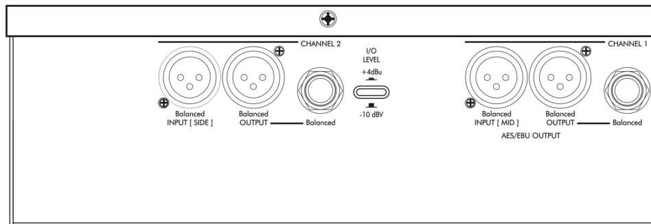
Figure 3 – Rear connections
