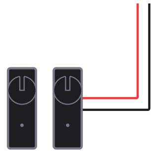
Entrapment Protection Sensor (Supplied by Gate Manufacturer)
