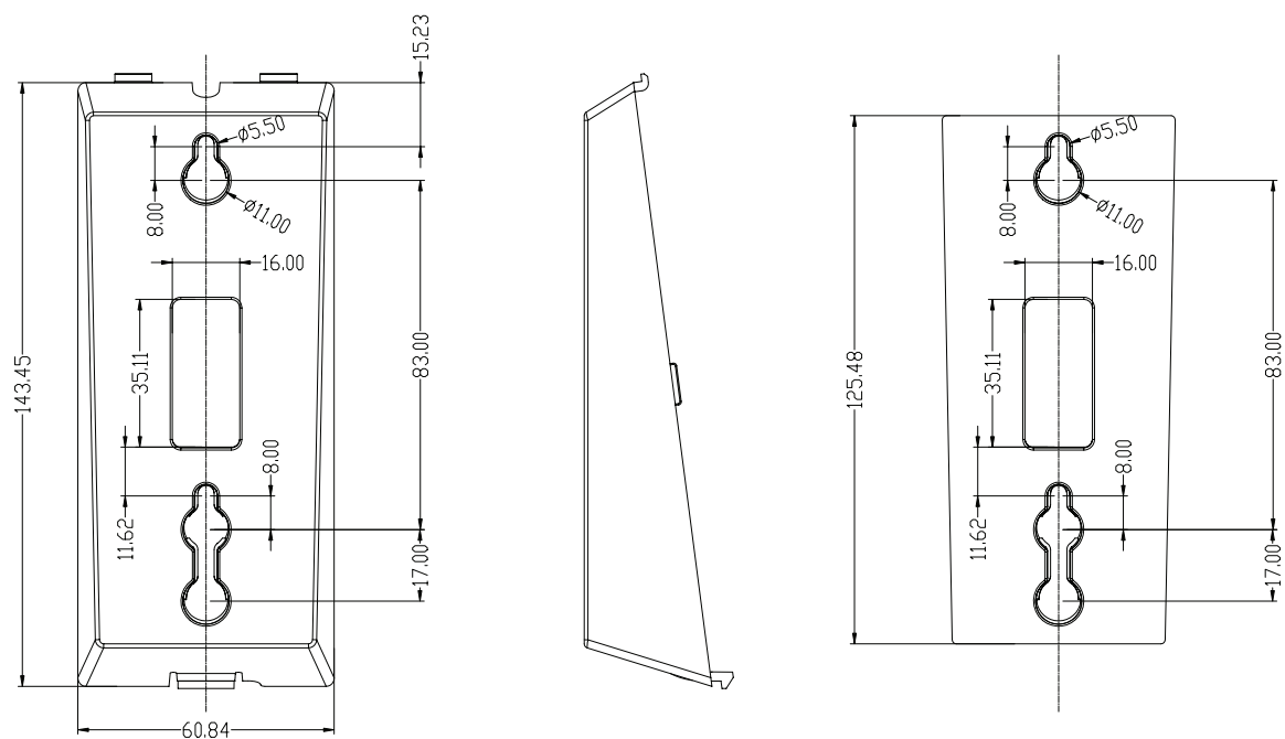
Single Drawing(Scale 1:1)
