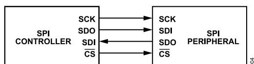
Figure 4. SPI Configuration
