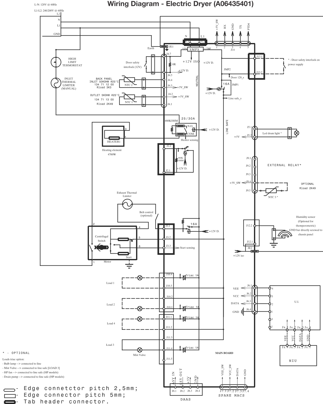
Wiring Diagram - Electric Dryer (A06435401)
