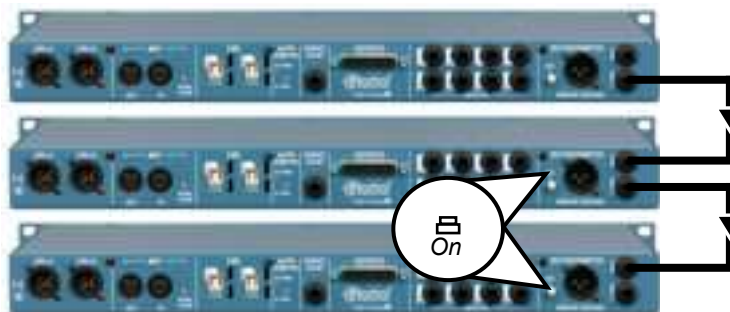
Linking multiple SW8-USB units using 1/4" TRS cables
