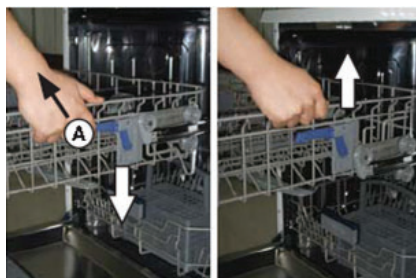
To lower position
