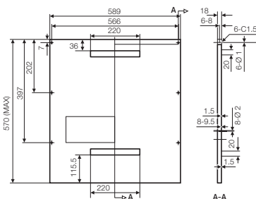
Semi built in
