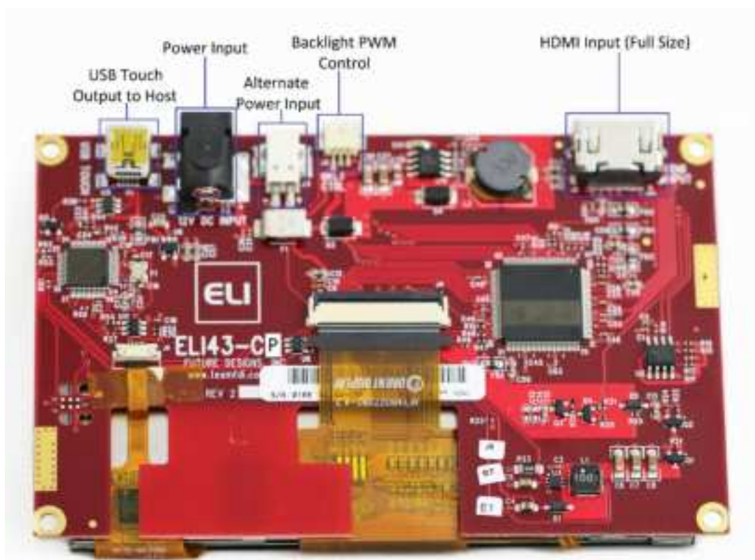
Figure 2. ELI43-CP Connectors
