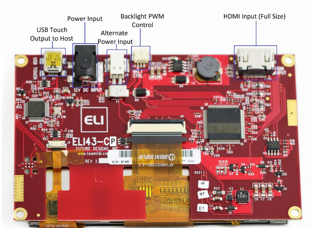
Figure 2. ELI43-CP Connectors
