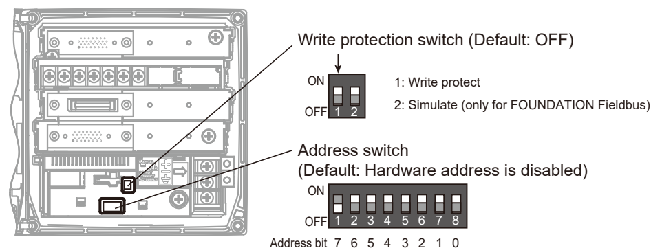
Figure 2.4 DIP switches
