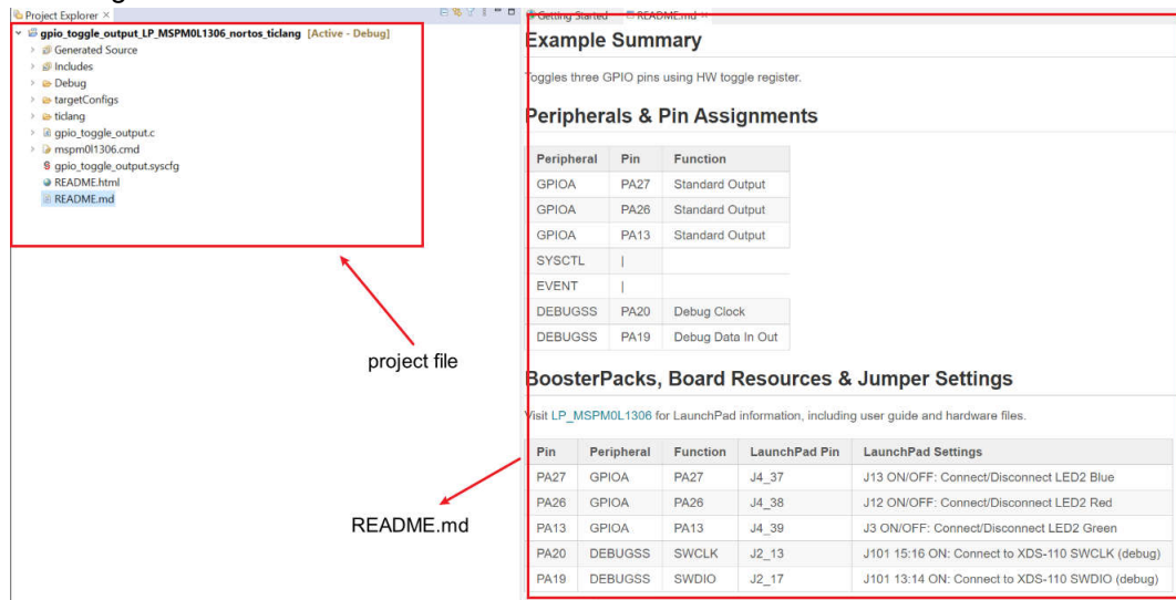
Figure 2-31. Project and README.md
