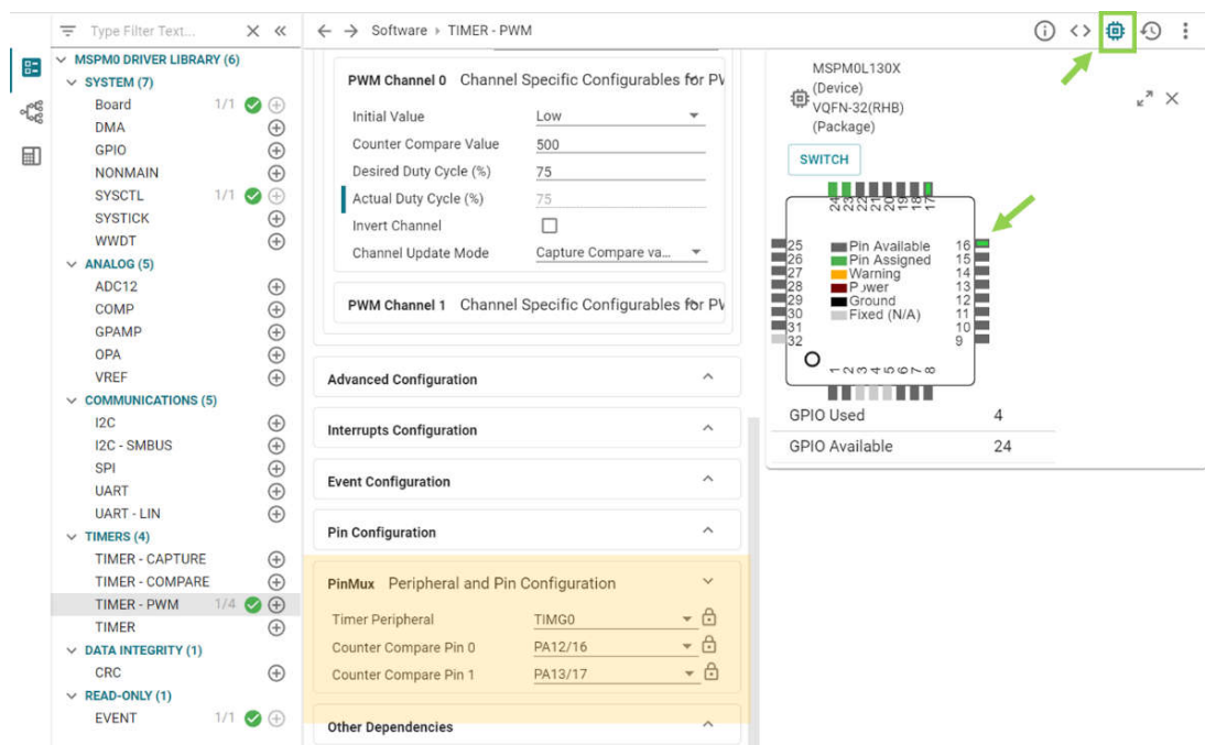
Figure 2-44. Pins Configuration
