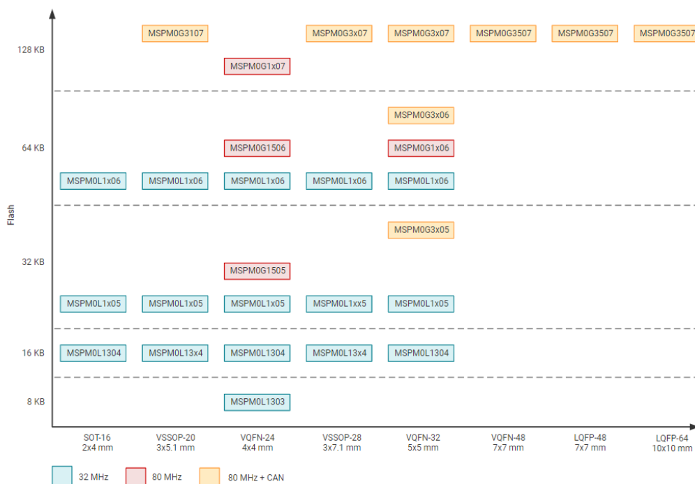
Figure 2-10. Portfolio of MSPM0L and MSPM0G Series
