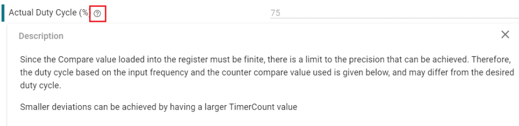
Figure 2-43. To Get Detailed Information of Each Item
