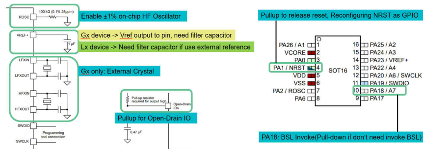
Figure 2-38. MSPM0 Minimum System Attention
