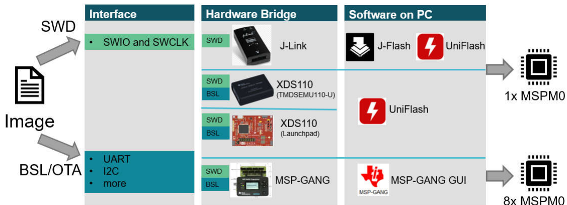
Figure 2-40. Program Software and Tool
